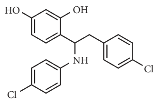
4-(2-(4-chlorophenyl)-1-((4-chlorophenyl)amino)ethyl)benzene-1,3-diol (CBED)
