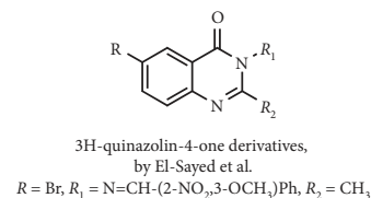
FIGURE 7: Structure of a 3H-quinazolin-4-one derivatives with XO inhibitory activity.
