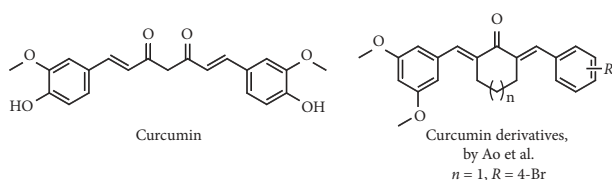
FIGURE 17: Structure of curcumin and analogues with XO inhibitory activity and decreasing effect of serum UA levels.
