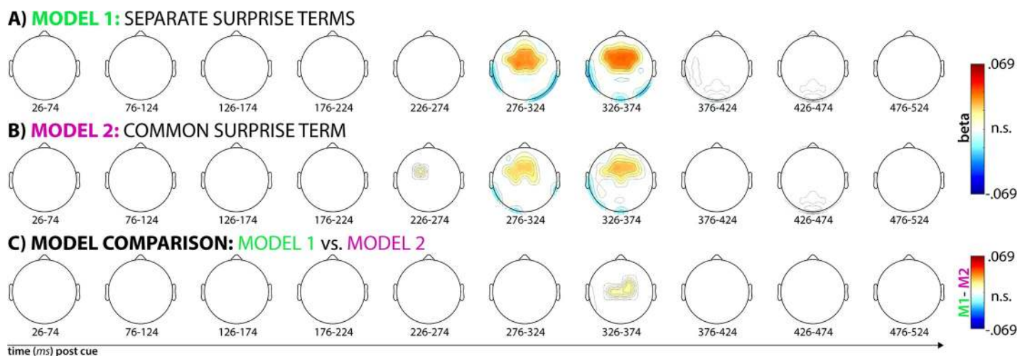
Fig 4. Results from the whole-brain single-trial model fitting analysis described in Fig 2. Each topography depicts the averaged standardized beta coefficient at each channel in the respective time window (x-axis) and model (plots A and B), as well as the M1-M2 model comparison (plot C). White areas denote channels at which the fit within the depicted time-window was non-significant ( p < .00044 ). In A and B, red areas denote significant positive correlations between the respective model and the EEG data, blue areas denote significant negative correlations. In C, red areas denote higher correlations between Model 1 and the data compared to Model 2.
