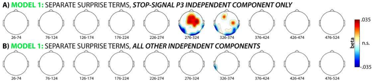
Fig 9. A) A reanalysis of the single-trial model fitting analysis for the winning model (separate surprise terms cf. Fig 4A) using just the one IC that was selected to reflect the stop-signal P3 in the merged dataset. The significant association between fronto-central EEG activity following unexpected cues in the CMO task and the surprise model is retained when the data is reconstructed solely using that one ICA (out of ~17.1 overall ICs that were extracted per subject on average). B) For comparison, no significant association was found when the data were reconstructed based on the ~16.1 ICs that did not reflect the stop-signal P3.
