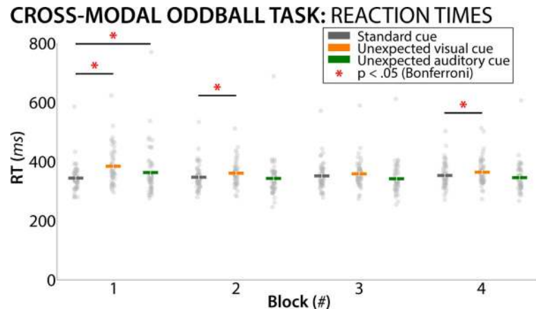
Fig 3. Reaction time data from the cross-modal oddball task. Significant individual comparisons (Bonferroni-corrected) are highlighted in red. For both unexpected auditory and unexpected visual cues, reaction times were slower compared to standard cues in Block 1. This effect wore off over time. White error bars denote the standard error of the mean, gray dots indicate individual subject condition means.
