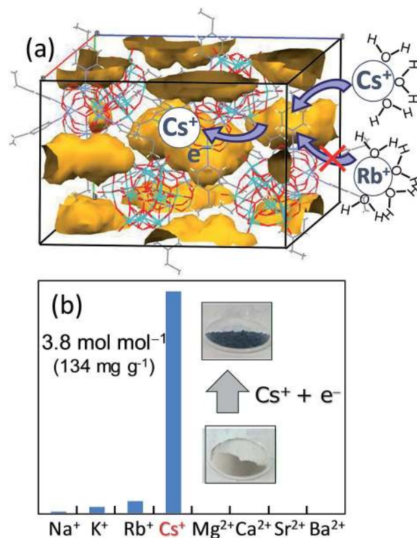
Fig. 8 (a) Crystal structure of (etpy)_2[Cr_3O(OOCH)_6(etpy)_3][\alpha\text{-SiMo}_{12}O_{40}] \cdot nH_2O ( etpy = 4\text{-ethylpyridine} ). Each void (in yellow-brown) has a size of ca. 6.5 \text{ \AA} \times 12.5 \text{ \AA} . (b) Amounts of cations incorporated by the reduction-induced method. Note that there is a color change due to the reduction of POM upon Cs^+ uptake. 63
