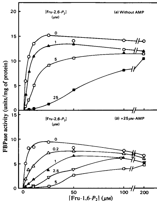
Fig. 7. Inhibition of FBPase by Fru-2,6- P_2 at various concentrations of substrate in the absence (a) and in the presence (b) of 25\mu\text{M} -AMP (From Van Schaftingen & Hers, 1981b.)
