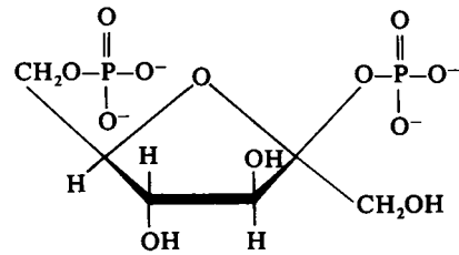
Fig. 2. \beta -Fructose 2,6-bisphosphate
