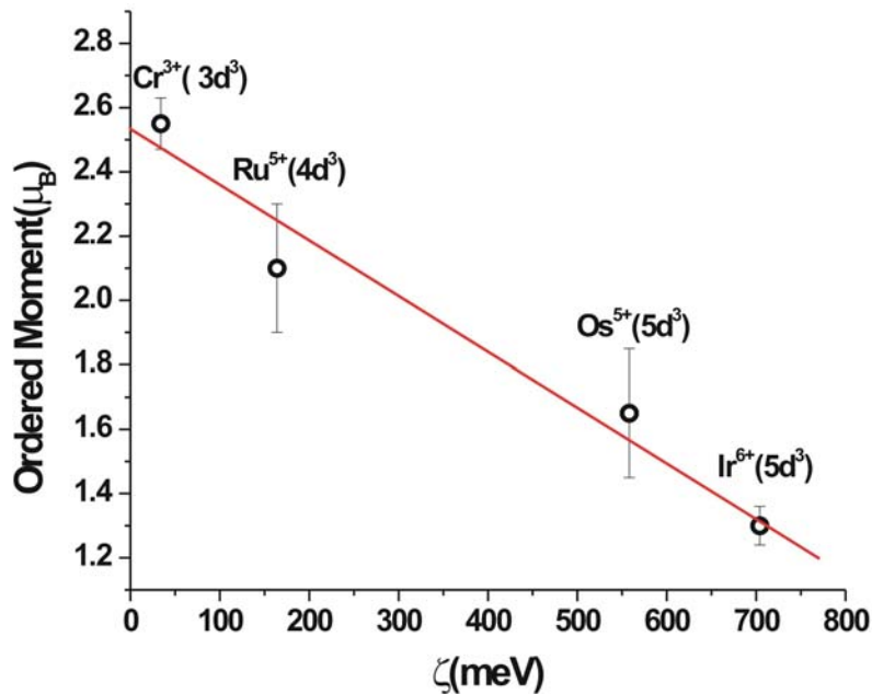
Figure 1. Correlation between the ordered moment measured by neutron diffraction and the free ion, one electron SOC constant for nd^3 ions in a perovskite environment. The error bars represent the spread of values indicated in Table 1. The SOC constants for \text{Ru}^{5+} , \text{Os}^{5+} and \text{Ir}^{6+} are extrapolated from C.-G. Ma and M.G. Brik, J. Lumin. 145 (2014) 402 and for \text{Cr}^{3+} from M. Blume and R.A. Watson, Proc. Roy. Soc. A270(1962) 127.
