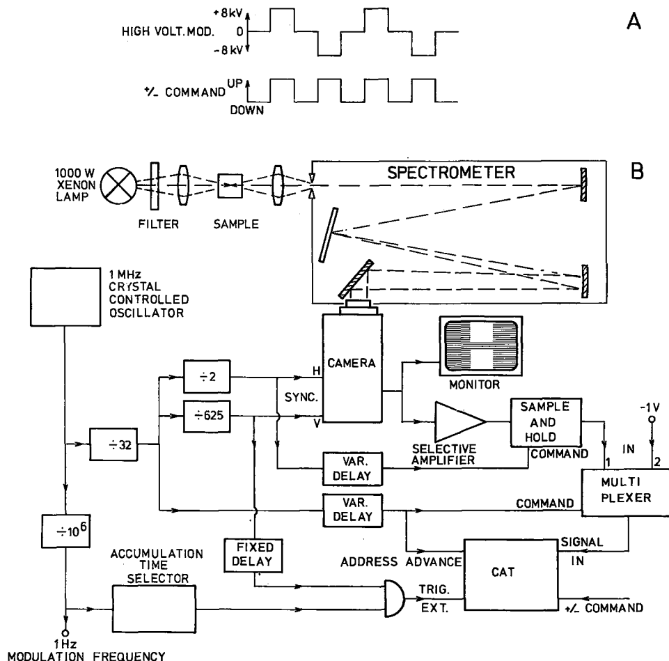
Fig. 1. (a) Wave forms used for obtaining the Stark modulation spectra. (b) Block diagram of the optical multichannel detection system.
