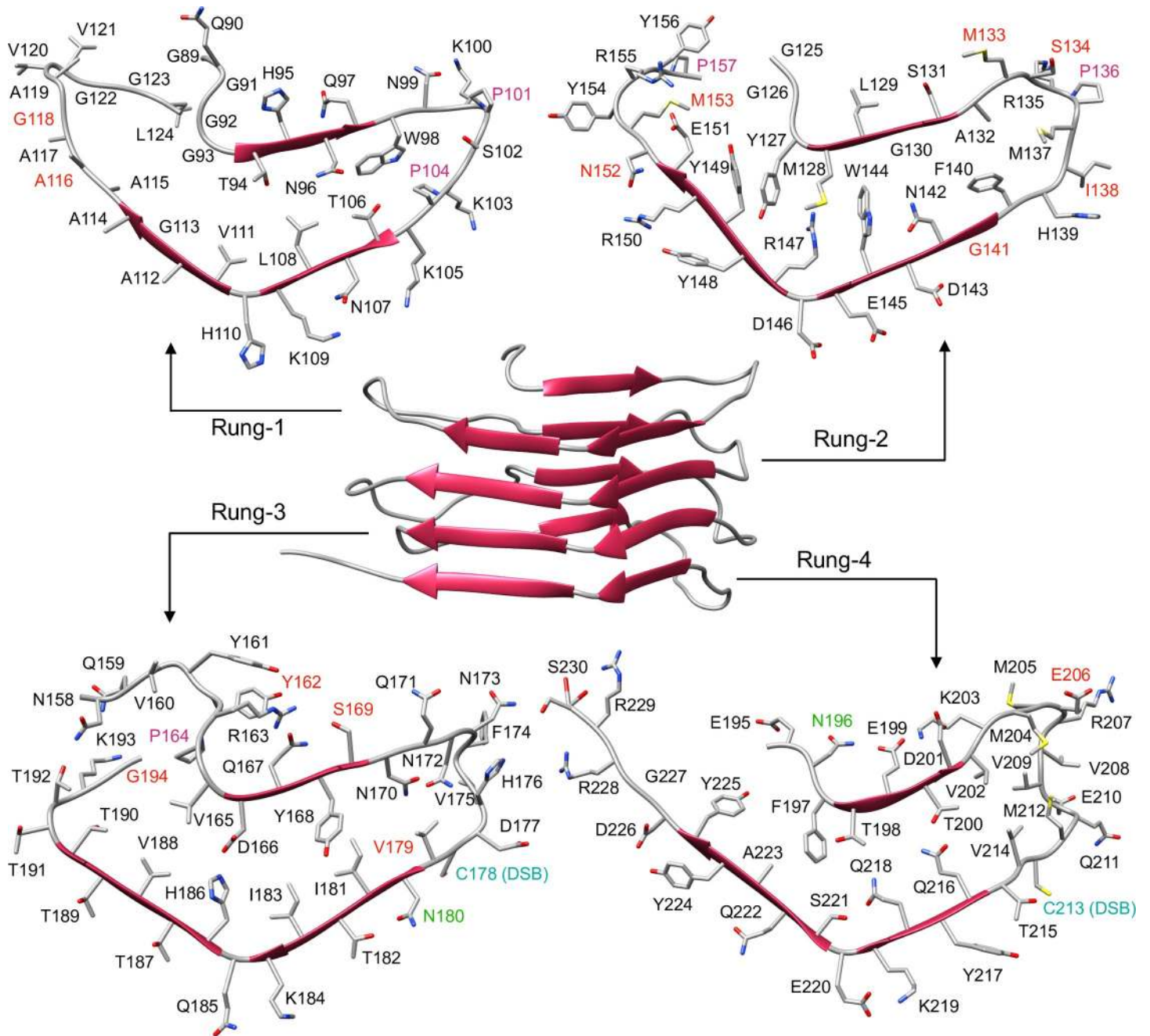
Fig 1. View of the 4RβS PrP Sc Model. The structure of PrP Sc modelled as a 4RβS (β-strands represented as red arrows) is depicted in the center of the figure. Residues are displayed in each individual rung (1–4) with different colors. PK cleavage sites identified by mass spectrometry in two different previous reports are colored in red [14] [15]. Glycosylation sites are labelled in green. Prolines are colored in purple. Cysteine is indicated in cyan.
