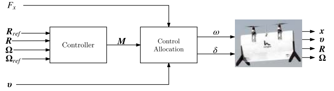
Fig. 10: The control structure of the proposed controller
