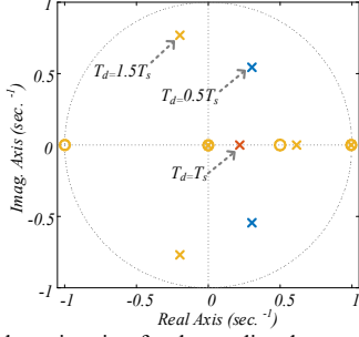
Fig. 12. Eigenvalue migration for the predicted computation delay T_{d,sp} = 0.5T_s, T_s, \text{ and } 1.5T_s .
