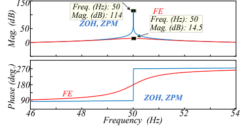
Fig. 17. Frequency response of the resonant controller using ZOH, ZPM and FE
