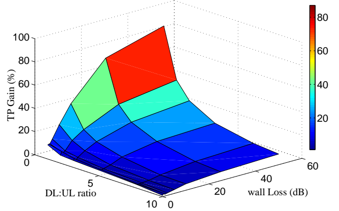
Fig. 2. TP gain of FD over HD vs. wall loss (dB) and DL/UL ratio for \rho_{AP} = 1 .
