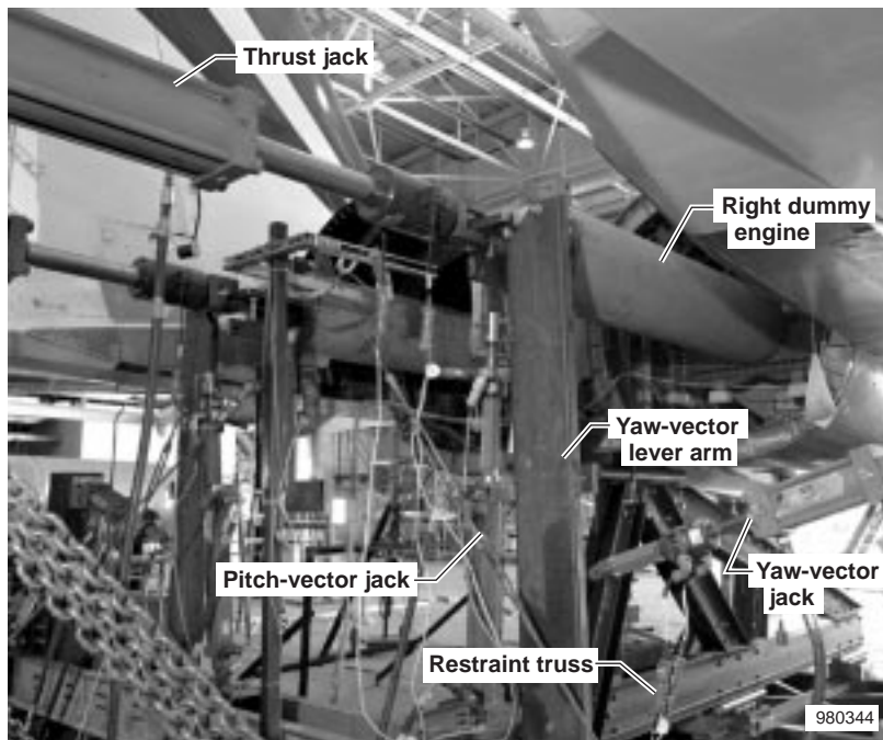
Figure 12. “Cold loads” test setup in the flight loads laboratory.
