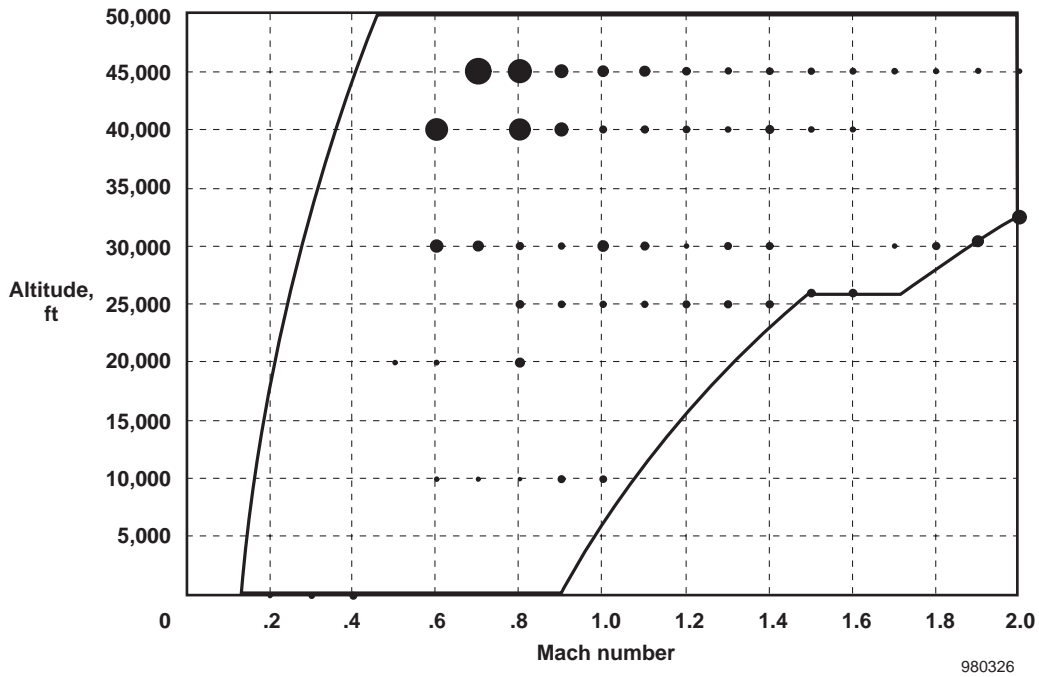
Figure 23. Relative change in percent difference in gross thrust between direct thrust-measurement technique and postflight model as a function of flight condition; maximum power.
