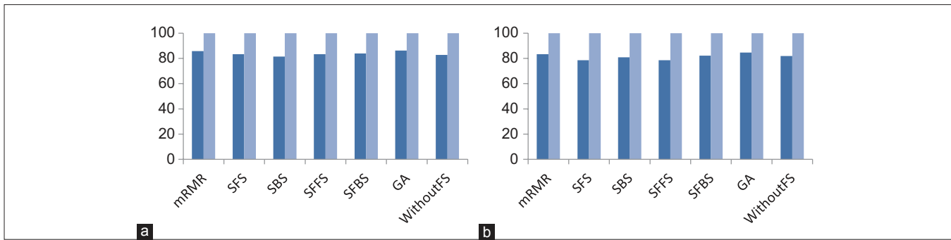
Figure 10: Comparison of the accuracy of different feature selection methods in 90° breast images. (a) Comparing results on right breast images; (b) comparing results on left breast images. (Dark blue: Mean accuracy, light blue: Max accuracy)
