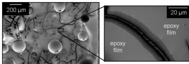
Figure 8. SEM of healed crack plane from an in situ sample with 80% epoxy-hexyl acetate capsules (15 wt% loading). The microcapsules have ruptured to produce an excessively thick epoxy film on the surface (shown in the inset) that prevents the crack faces from joining to heal the epoxy.
