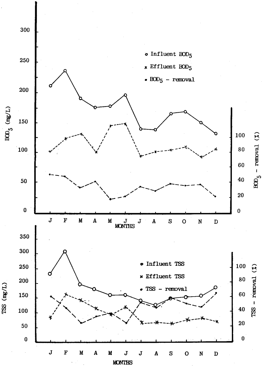
Fig. (2) - Monthly Performance of Primary Settling Tanks
