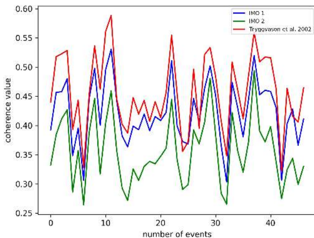
Figure 4. Coherence values for the three velocity models. The Tryggvason et al. (2002) model shows the best values of coherence.
