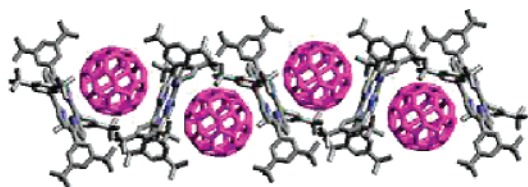
FIGURE 2. Zigzag alternating C_{60} and H_2TTP moieties in H_2T_{3,5}\text{-di-}t\text{-butylPP}\cdot C_{60} . 6 Solvate molecules have been omitted for clarity.
