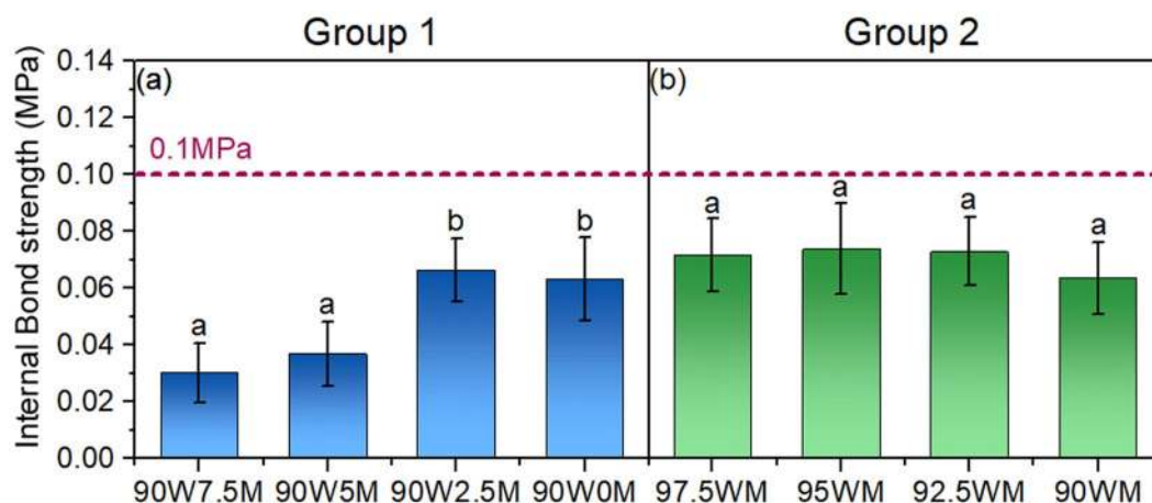
Figure 7. The internal bond strength of Group 1 (a) and Group 2 (b). The horizontal line indicates the minimum value of the internal bond strength required to meet the ANSI A208.1 standard for LD-1 grade 6 . In each figure, columns with common letters are not significantly different at 95% confidence level ( p -value > 0.05 ).
