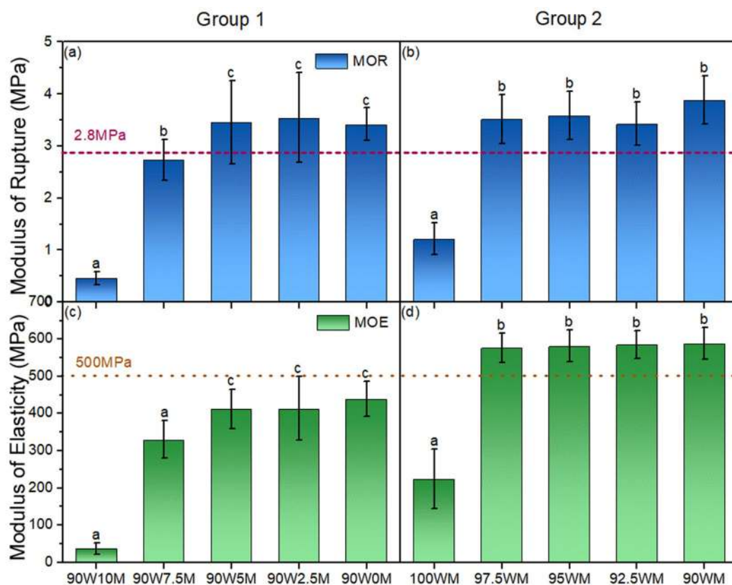
Figure 6. The modulus of rupture (a,b) and the modulus of elasticity (c,d) of Group 1 (a,c) and Group 2 (b,d). The horizontal lines indicate the minimum value of the modulus of rupture and the modulus of elasticity required to meet the ANSI A208.1 standard for LD-1 grade 6 . In each figure, columns with common letters are not significantly different at 95% confidence level ( p -value > 0.05 ).
