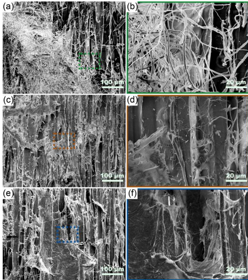
Figure 8. SEM images of different mixtures of raw materials with different magnifications, 200\times (a,c,e) and 1000\times (b,d,f). (a,b) 90% Wood + 10% Mycelium; (c,d) 90% Wood-Mycelium + 2.5% CNF; (e,f) 90% Wood + 10% CNF.
