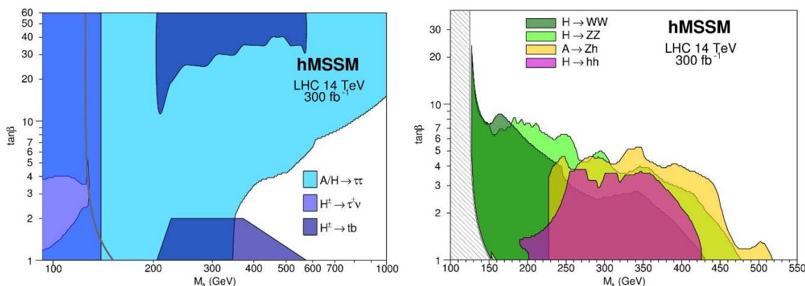
Figure 14. Projections for the LHC with \sqrt{s} = 14 \text{ TeV} and 300 \text{ fb}^{-1} data for the 2\sigma sensitivity in the h\text{MSSM} [\tan \beta, M_A] plane from the search for A/H^\pm states in their fermionic decays (left) and A/H states in their bosonic decays (right). The same color code as at \sqrt{s} = 8 \text{ TeV} has been used and, for the fermionic channels, we add a constraint from the H^+ \rightarrow tb mode depicted in dark blue.
