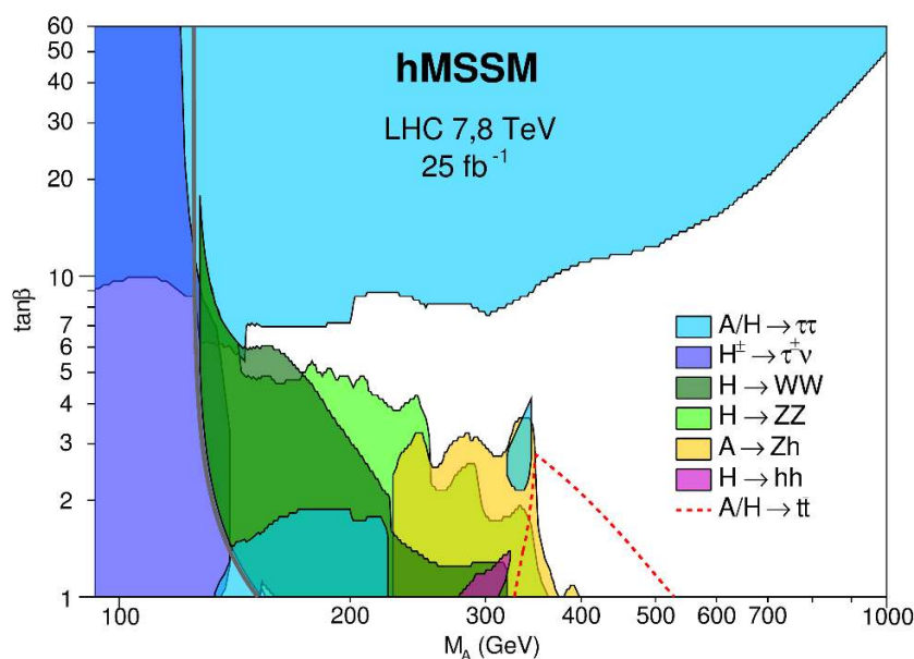
Figure 18. Expectations for the 2\sigma sensitivity in the hMSSM [\tan \beta, M_A] plane when the searches for the A/H/H^\pm states in all channels, including the gg \rightarrow H/A \rightarrow tt process, are combined at the LHC with \sqrt{s} = 8 TeV and 25 \text{ fb}^{-1} data.
