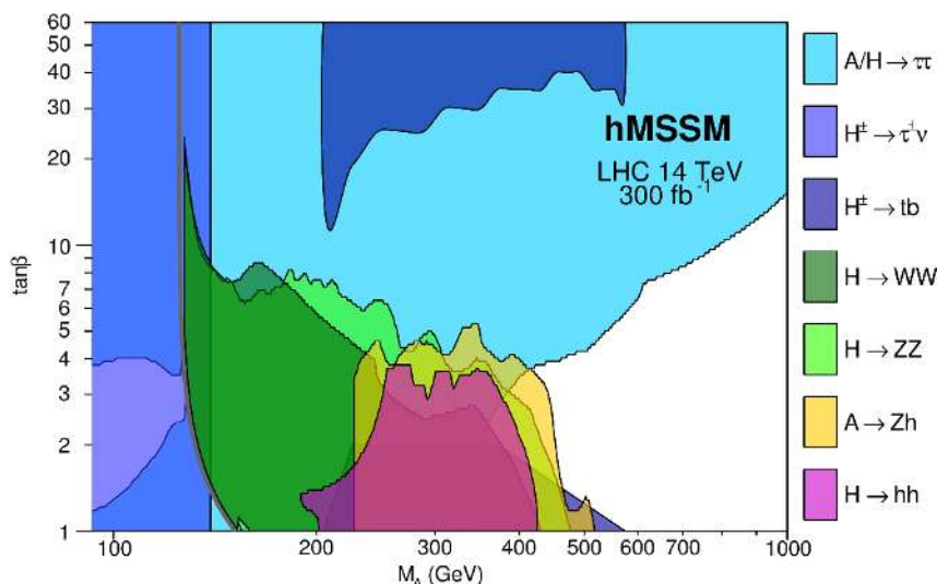
Figure 15. Projections for the LHC with \sqrt{s} = 14 \text{ TeV} and 300 \text{ fb}^{-1} data for the 2\sigma sensitivity in the h\text{MSSM} [\tan \beta, M_A] plane when the searches for the A/H/H^\pm states in their fermionic and bosonic decays are combined.
