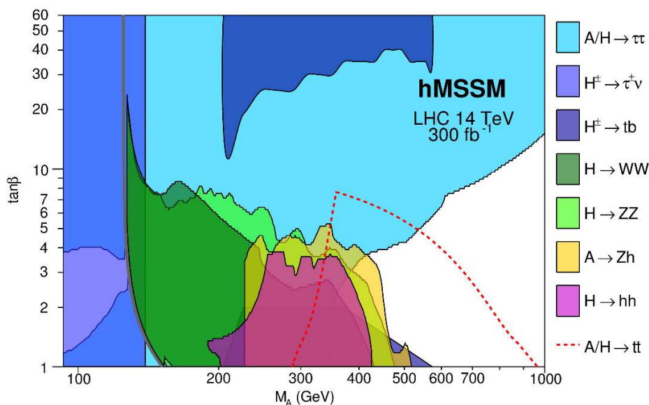
Figure 19. The same as in figure 18 but at the LHC with \sqrt{s} = 14 TeV and 300 \text{ fb}^{-1} data.
