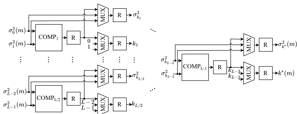
Figure 7. Architecture of the OTM.
