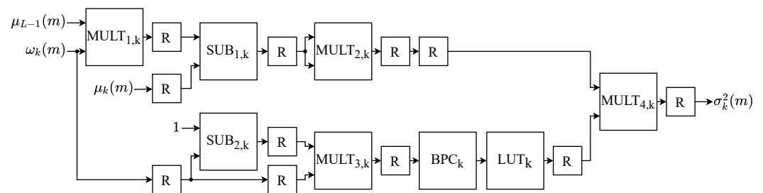
Figure 6. Architecture of the BCV_k submodule.
