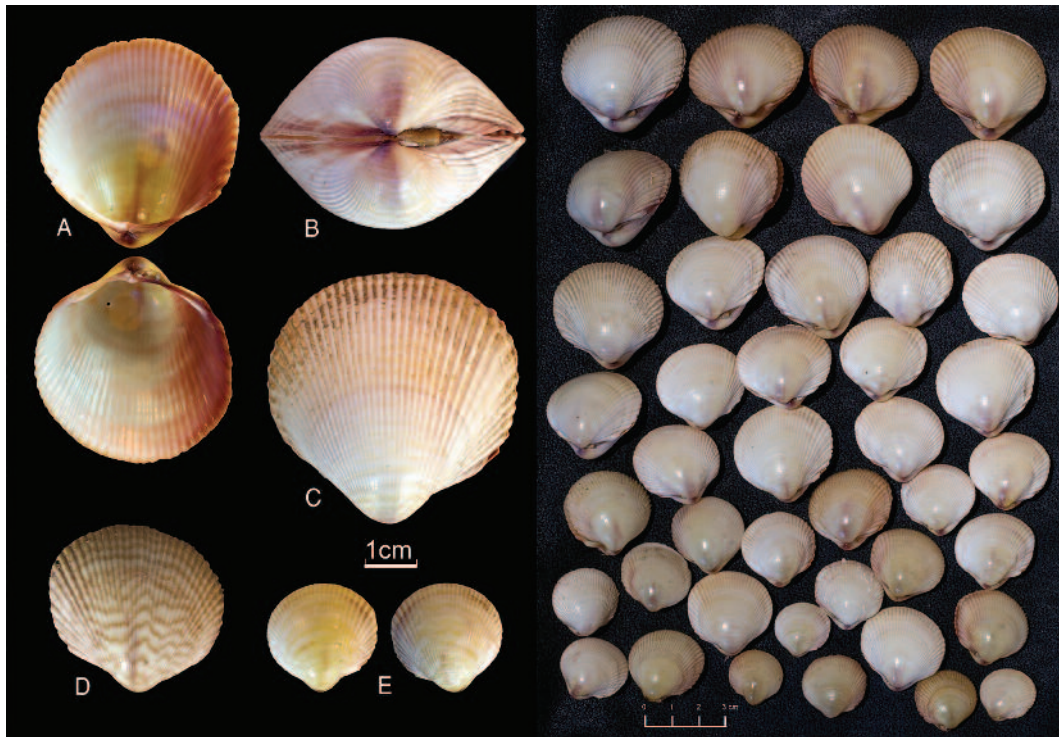
FIG. 2. Fulvia fragilis (Forsskal in Niebuhr, 1775). A: interior, B: umbilical view of the biggest individual found, C: biggest individual found measuring 44×44 mm, D: single valve with particular indented pattern, E: smallest individual found measuring 17×17 mm. On the right, a portion of the bivalves found and kept in author's collection.
