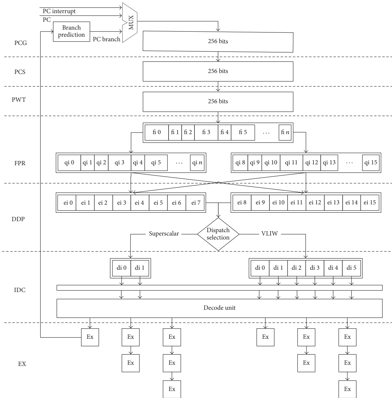
FIGURE 5: Universal pipeline structure for fused microarchitecture.
