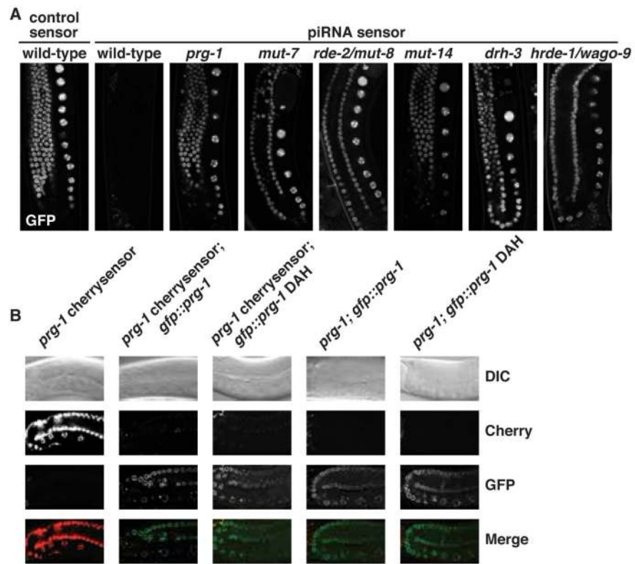
Fig. 2. A specific endo-siRNA pathway acts downstream of and is required for piRNA-mediated silencing. (A) piRNA sensor expression in siRNA pathway mutants as in Fig. 1A. (B) A second 21UR-1 piRNA sensor strain (cherrysensor) expressing mCherry-H2B in prg-1 ( n4357 ).
