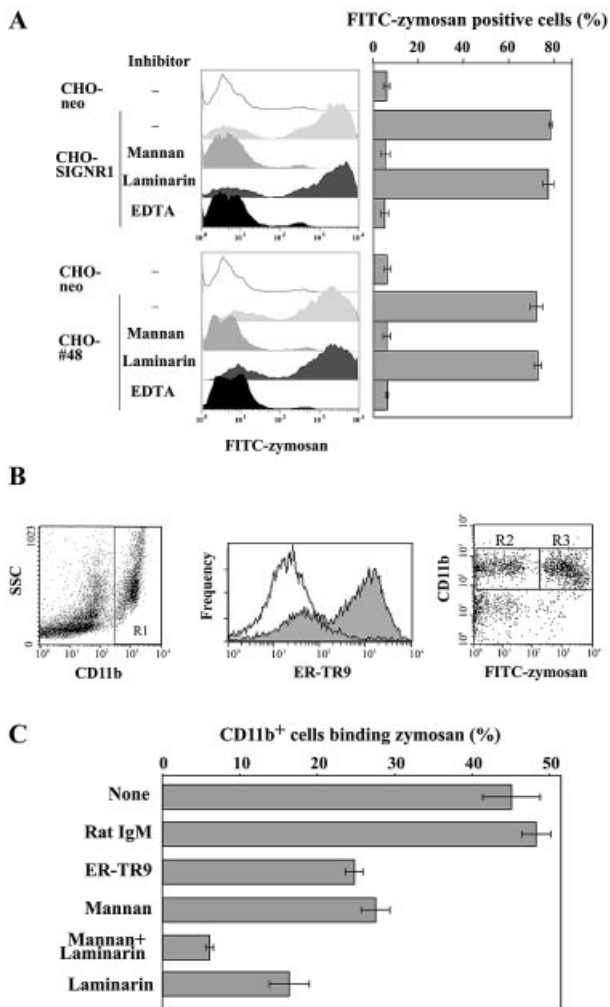
Fig. 5. Direct binding of stably SIGNR1-transfected CHO cells and of resident peritoneal cells expressing SIGNR1. (A) SIGNR1 itself bound FITC-zymosan in a mannan and EDTA-sensitive manner. CHO-SIGNR1 and CHO-#48 cells lacking the cytoplasmic tail of SIGNR1 were incubated with FITC-zymosan on ice with/without inhibitors described. Reduction of FITC-zymosan capture by inhibitors is depicted in the right panel. (B) Expression of SIGNR1 on resident peritoneal cells was analyzed by flow cytometry. A majority of CD11b + cells were stained with ER-TR9, anti-SIGNR1 mAb (left and center panels). Open histogram represents control staining with DX-5 antibody. The CD11b + cells were capable of binding FITC-zymosan at 4°C (right panel). (C) Cooperation in zymosan binding by SIGNR1 and laminarin-sensitive receptor. Peritoneal cells were pretreated with inhibitors represented for 1 h. Binding (%) indicates the percentage of FITC + cells in CD11b + cells.
