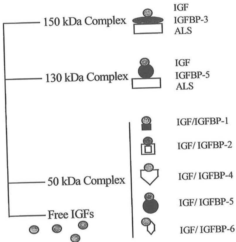
Fig. 1: IGFs (IGF-I or -II) in human serum (proposed model) (RAJARAM et al., 1997; TWIGG and BAXTER, 1998) (IGFs (IGF-I oder -II) im menschlichen Serum (vorgeschlagenes Modell))
