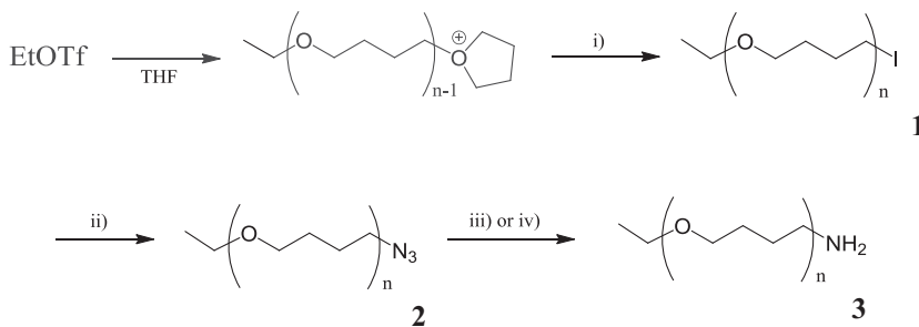
Scheme 2. One-pot preparation of amino-terminated PTHF. i) NaI (4 equiv.), 1 h (quant.); ii) \text{NaN}_3 (5 equiv. from a 150 mg \text{mL}^{-1} water aqueous solution), reflux overnight (quant.); iii) Pd/C 10% (54.4 mg \text{mmol}^{-1} of EtOTf), \text{H}_2 atm, overnight (yield: 90%); iv) \text{PPh}_3 (7 equiv.), reflux 3 h (yield: 95%).
