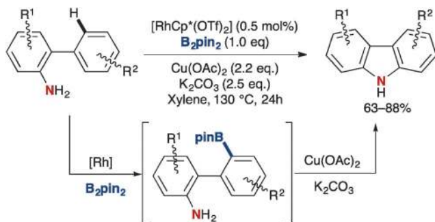
Scheme 24 'One pot' borylation-amination procedure for the synthesis of carbazoles.
