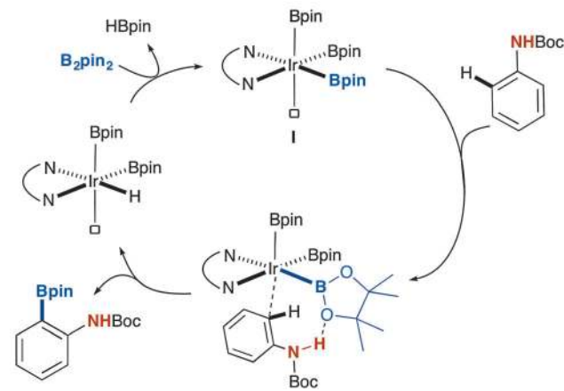
Scheme 16 Outer-sphere directed borylation of Boc-protected anilines and enamines.
