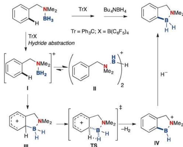
Scheme 27 N-directed borylation via borenium intermediates.
