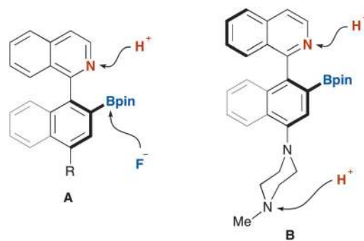
Fig. 1 Borylated aryl isoquinoline (BAI) dyes.
