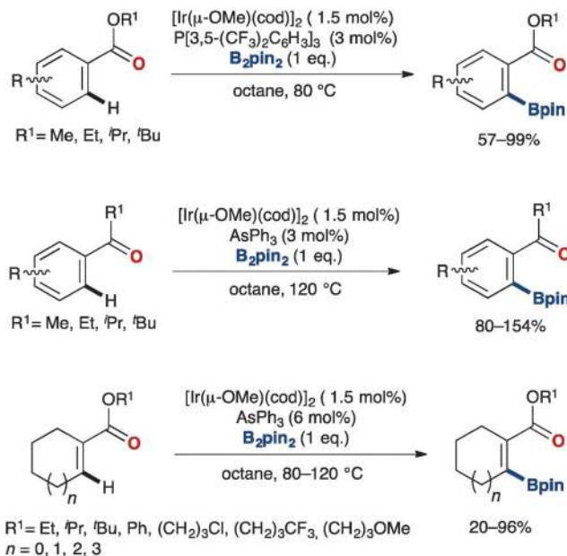
Scheme 4 Oxygen-directed Ir-catalysed borylations.
