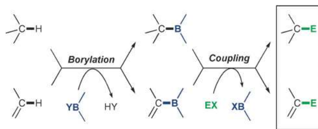
Scheme 1 Functionalization of hydrocarbons via direct borylation/cross-coupling strategies.
