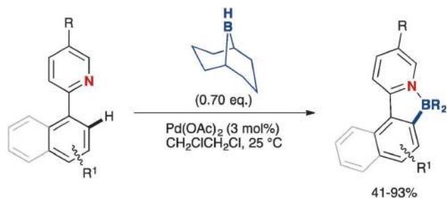
Scheme 22 Pd-catalysed C-H borylation of 2-arylpyridines.
