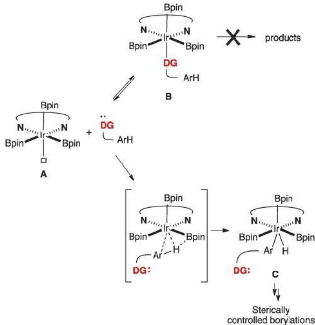
Scheme 3 Analysis of regioselectivity in Ir-catalyzed borylations.
