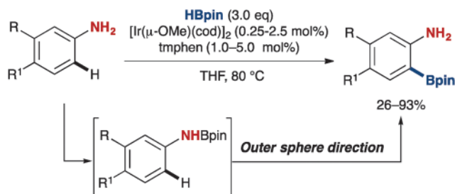
Scheme 17 Outer-sphere directed borylation of free anilines.
