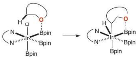
Scheme 31 Site selective \beta -borylation of cyclic ethers.
