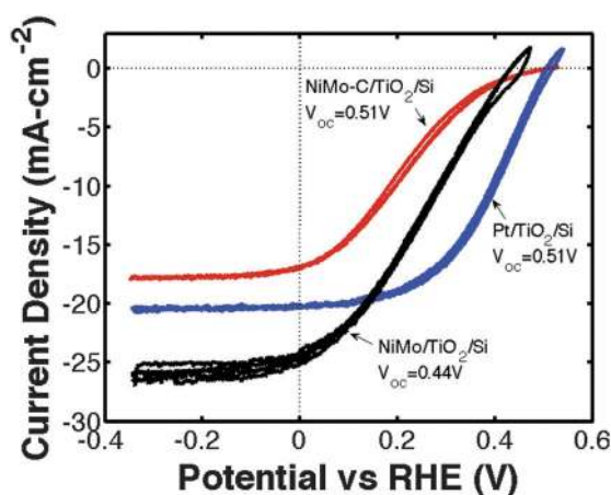
Fig. 9 Current-density versus potential ( J – E ) behavior for three samples in 1.0 \text{ M H}_2\text{SO}_4(\text{aq}) , demonstrating the decrease in open-circuit voltage ( V_{\text{oc}} ) consistently observed in the Ni–Mo containing samples as compared to in samples that were coated with Pt. A V_{\text{oc}} similar to that exhibited by the Pt-coated Si microwire arrays was observed upon introduction of a carbon-supported Ni–Mo catalyst that did not require annealing to activate the Ni–Mo after deposition.
