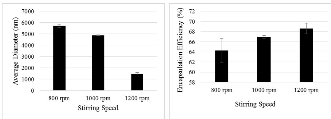
Figure 21. Graphs showing effect of stirring rate on average diameter (left) and Encapsulation Efficiency (right)
