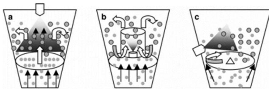
Figure 2. Schematics of a fluid-bed coater. (a) Top spray; (b) bottom spray; (c) tangential spray
