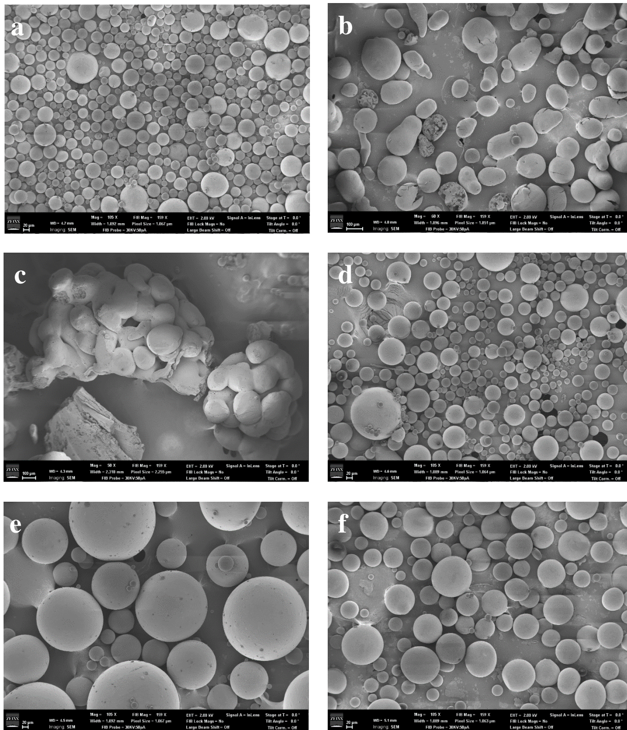
Figure 10. SEM micrographs of PMMA-dye microcapsules
