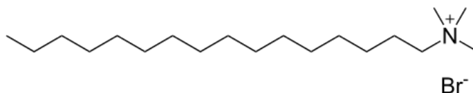
Figure 7. Chemical structure of Cetrimonium Bromide (CTAB)
