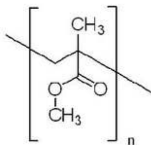
Figure 5. Chemical structure of poly (methyl methacrylate) (PMMA)
