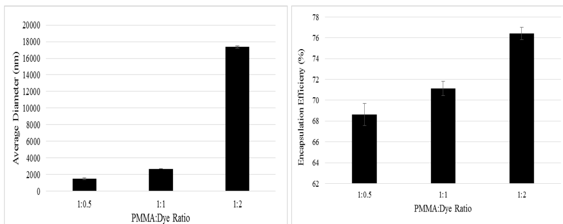
Figure 16. Graphs showing effect of dye content variation on average diameter (left) and Encapsulation Efficiency (right)
