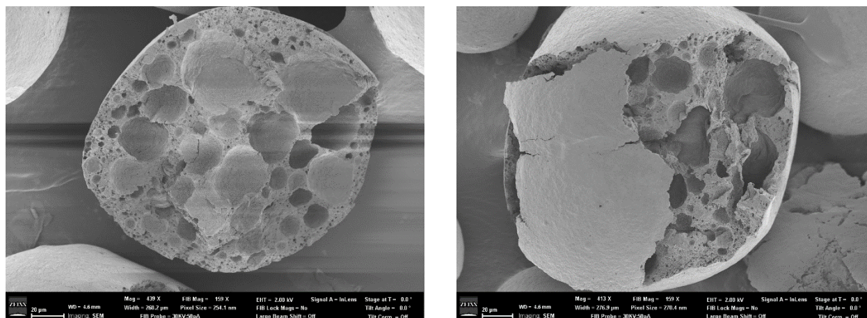
Figure 11. SEM showing interior structure of fractured microcapsules.
