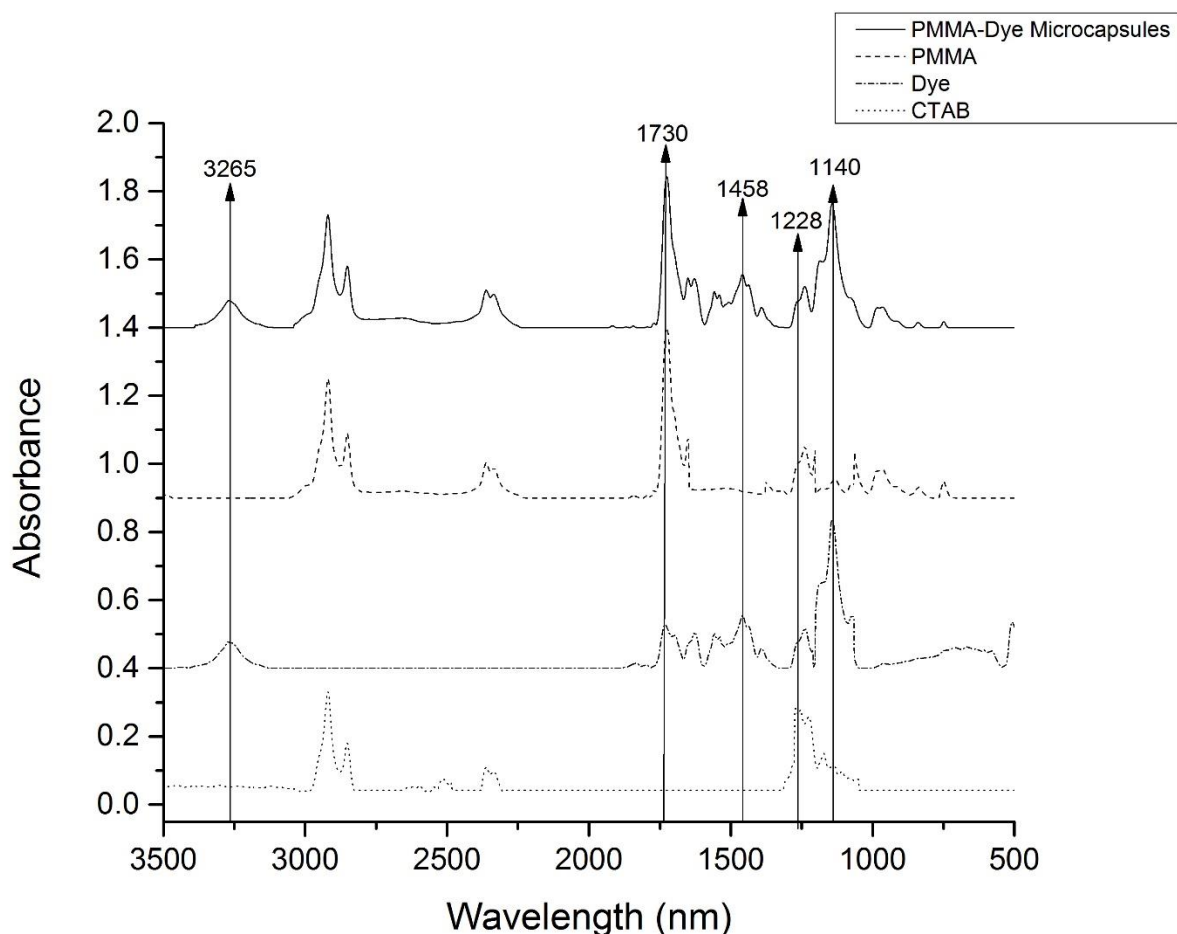
Figure 24. FTIR spectra of Dye, CTAB, PMMA and PMMA-dye Microcapsules.
