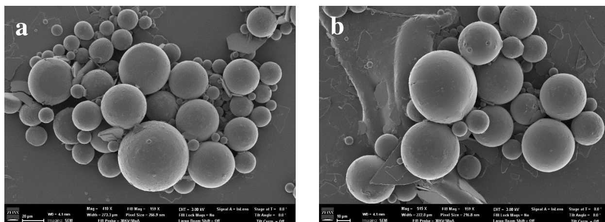
Figure 9. SEM micrographs of PMMA:Dye microcapsules ((a) 420x magnification & (b) 515x magnification)
