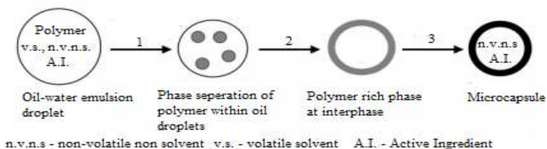
Figure 3. Schematic diagram of the shell formation mechanism (redrawn from [22] )
