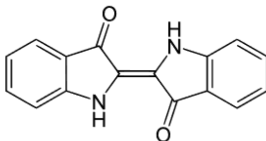
Figure 6. Chemical Structure of Indigo Dye
