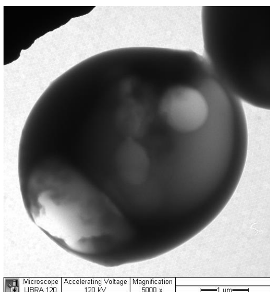
Figure 19. TEM image showing interior of PMMA-dye microcapsule synthesized at 40 °C.
