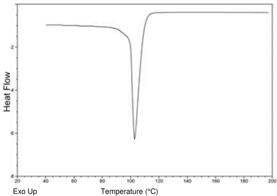
Figure 22. DSC to showing evaporation temperature of liquid indigo dye
