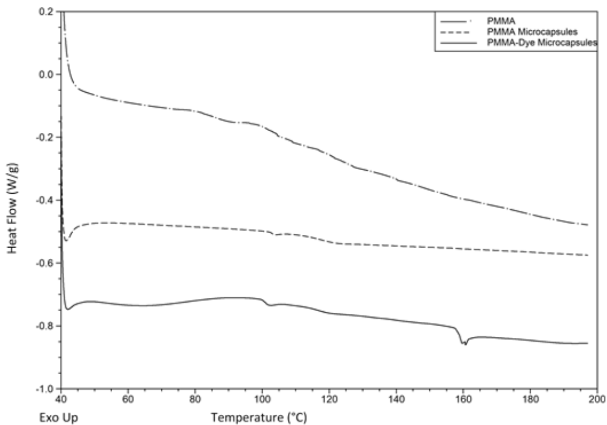
Figure 23. Thermal behavior of PMMA, PMMA microcapsules and PMMA-dye microcapsules.
