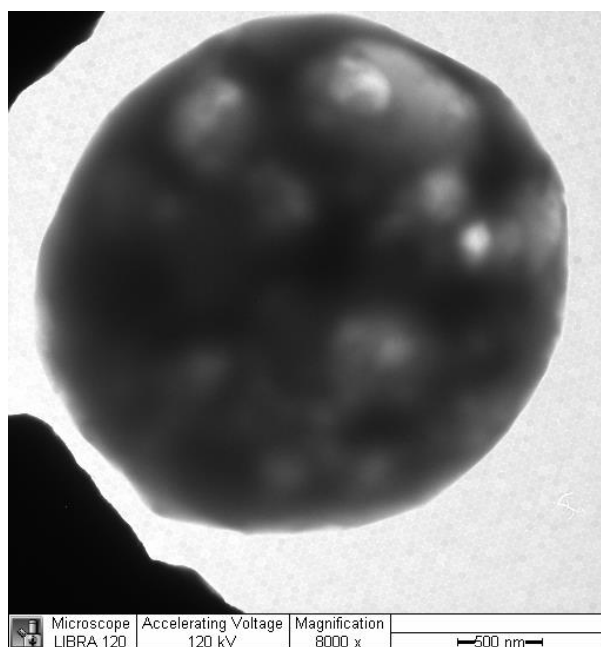
Figure 12. TEM image showing multi internal cavities
