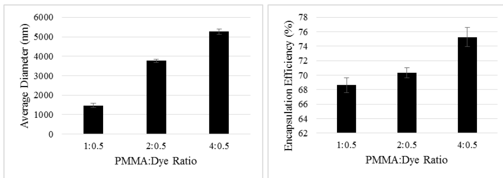
Figure 14. Graphs showing effect of PMMA:Dye Ratio on Average diameter (left) and Encapsulation Efficiency (right)
