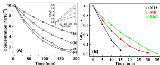
Figure 5. Photocatalytic degradation efficiency of: (A) MB using bare BiVO 4 (a) and BiVO 4 /CuCr 2 O 4 composites with ratio of 1:1 (b), 1:0.25 (c) and 1:0.0625 (d) (inset of figure shows their respective kinetic fit curves for dye degradation) [129]; and (B) MO, MB and RhB with Ag 2 CO 3 under visible light illumination with 400 nm [133] (Reproduced with permission from [129] copyright RSC publications and [133] copyright from Elsevier).
