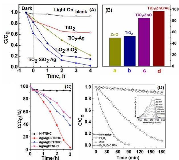
Figure 4. Photocatalytic degradation of: (A) RhB without any catalyst and with TiO 2 , TiO 2 -Ag, TiO 2 -SiO 2 and TiO 2 -SiO 2 -Ag as the catalysts under visible light [41]; (B) MO over different catalysts for 30 min under UV light [121]; (C) MO by different silver/silver halides/titanate films under visible light illumination [123]; and (D) MB in the presence and absence of nano-adsorbents (inset shows the time-dependent absorption spectra of MB degradation over Fe 3 O 4 -ZnO [40] (Reproduced with permission from [41,123] copyright American Chemical Society Publications; [121] copyright Elsevier and [40] copyright RSC publications).
