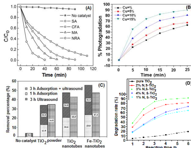
Figure 3. Photocatalytic degradation of: (A) MB with different nanostructures: spherical assemblies (SAs), nano-rod assemblies (NRAs), cauliflower-like assemblies (CFAs) and mushroom-like assemblies (MAs) of ZnO under UV light [78]; (B) resazurin by pure ZnO and Cu-doped ZnO photocatalyst with different Cu doping concentrations [80]; (C) dyes in the absence and presence of different \text{TiO}_2 -based catalysts under ultrasonic irradiation [86]; and (D) MO by N- and S-doped \text{TiO}_2 with different contents at pH 4 under sunshine irradiation [107] (Reproduced with permission from [78] copyright RSC publications and [80,86,107] copyright Elsevier).
