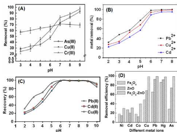
Figure 2. (A) Removal of 50 mg L -1 of As(III), Cu(II) and Cr(III) by 500 mg L -1 of Fe 3 O 4 -SiO 2 -poly(1,2-diaminobenzene) at 30 °C [61]; (B) removal of Cu (II), Pb(II) and Cd(II) by Fe 3 O 4 @SiO 2 @meso-SiO 2 -NH 2 microspheres at different pHs [62]; (C) % recovery of metal ions by Fe 3 O 4 /SiO 2 /Schiff base sorbent at different pHs [64]; and (D) removal of metal ions by Fe 3 O 4 , ZnO and Fe 3 O 4 -ZnO composites [40] (Reproduced with permission from [61,62, 64] copyright Elsevier and [40] copyright RSC publications ).
