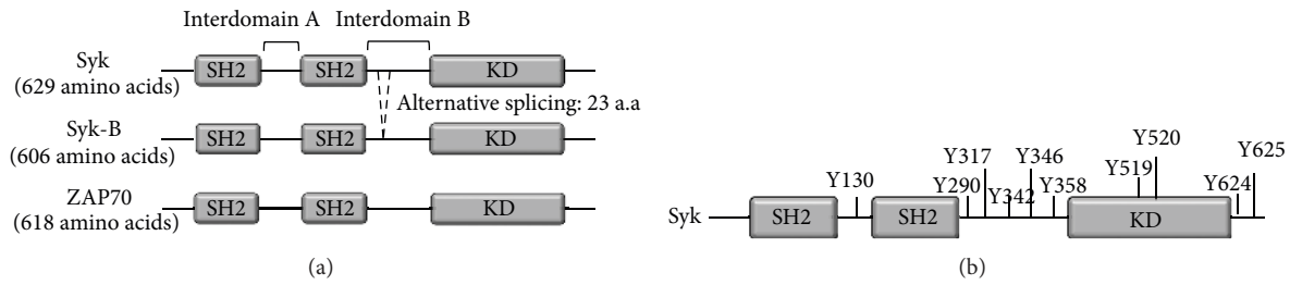
FIGURE 1: Biochemical features of Syk. (a) Structure comparison of Syk family kinases. (b) Phosphorylation sites of Syk.
