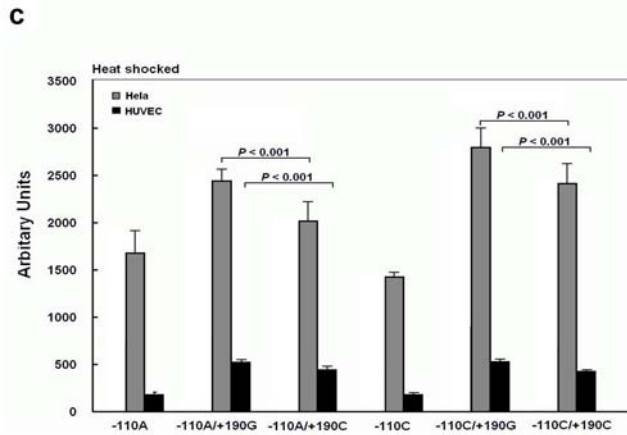
Figure 1. Effects of -110A/C and +190G/C polymorphisms on luciferase activity. (a), Schematic representation of HSPA1A gene 5' flanking region and reporter constructs. (b) to (c), the six reporter constructs and empty pGL3-Basic was transfected into HeLa and HUVEC cells under normal culture (b) or heat shocked conditions (c). All constructs were cotransfected with pRL-SV40 to standardize the transfection efficiency. Fold increase of luciferase activity was measured by defining the activity of the empty pGL3-Basic vector as 1. The RLA values are presented as means, and the T bars represent standard deviations (SD). Mean \pm SD from triplicates. doi:10.1371/journal.pone.0004851.g001
