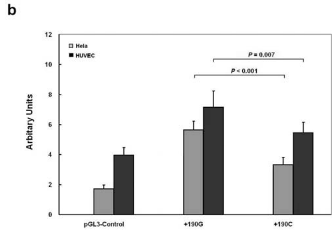
Figure 2. Effect of +190G/C polymorphism on the expression of luciferase. (a), Schematic representation of reporter constructs. (b), These constructs and empty pGL3-Control plasmid were transfected into HeLa and HUVEC cells. All constructs were cotransfected with pRL-SV40 to standardize the transfection efficiency. RLA was determined 24 hours later in normal culture condition. The RLA values are presented as means, and the T bars represent standard deviations (SD). Mean \pm SD from triplicates. doi:10.1371/journal.pone.0004851.g002
