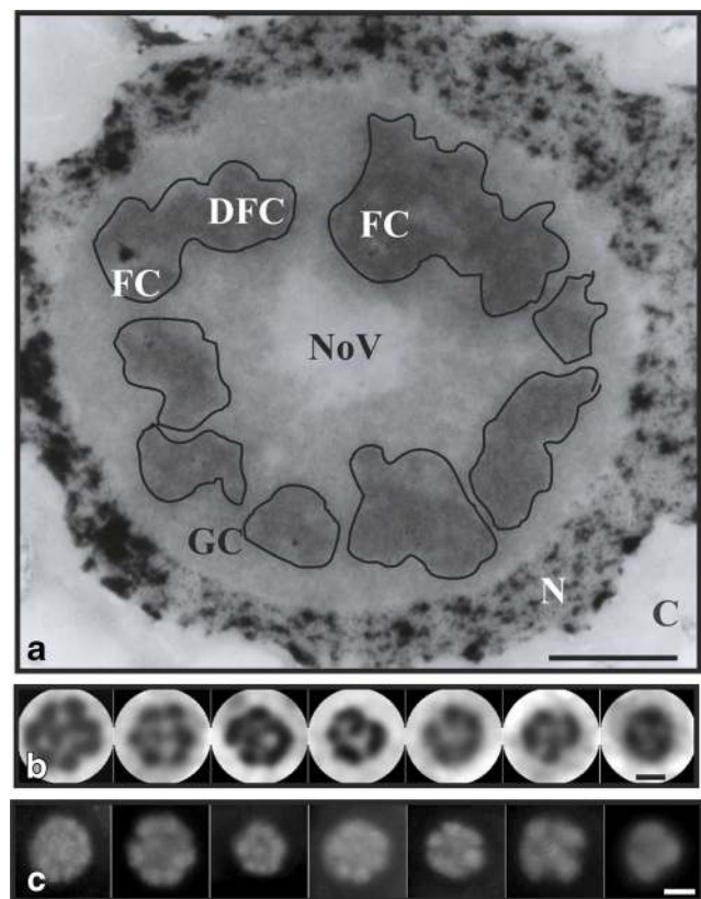
Fig. 2 Plant nucleolonema. Ultrastructure of a plant nucleolus with clearly visualized nucleolonema (dark nucleolar areas encircled with lines); modified NAMA-Ur technique (a). Scale bar, 2 \mu m. Nucleoli impregnated with silver nitrate; circular-shaped areas as nucleolonema units; the number and sizes of the units are correlated with nucleolar transcriptional activity, the greater number and bigger units, the more active nucleolus (b). Scale bar, 5 \mu m. Immunofluorescent identification of fibrillar protein, one of the key nucleolar protein and main protein component of nucleolonema as well as a marker of dense fibrillar component; circular areas correspond to those obtained with silver impregnation, their number and sizes also correspond to nucleolar activity (c). Scale bar, 5 \mu m. FC fibrillar centre, DFC dense fibrillar component, GC granular component, NoV nucleolar vacuole, N nucleus, C cytoplasm
