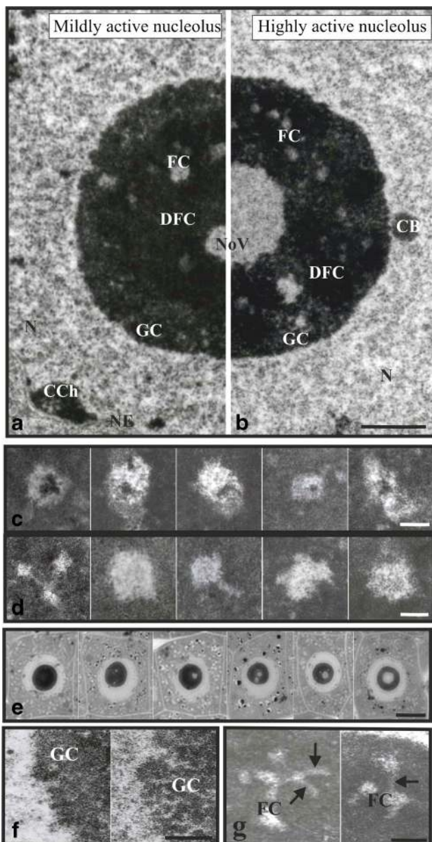
Fig. 1 Typical plant nucleoli of tip root meristem cells and nucleolar components. Ultrastructure of nucleoli, representing four-component morphology, i.e., fibrillar centres (FC), dense fibrillar component (DFC), granular component (GC), and nucleolar vacuoles (NoV); conventional electron microscopy technique images (a, b). A nucleolus with mild transcriptional activity; it is characterized by lower number of FCs and small NoV (a). A nucleolus with high transcriptional activity with greater number of FCs and big, centrally located NoV (b). Scale bar, 2 \mu m. Examples of different size and shape FCs (c, d); heterogeneous FCs containing clumps of condensed chromatin (c). Scale bar is 0.5 \mu m. Homogenous FCs (d). Scale bar, 0.5 \mu m. Tip root meristematic cells with nucleoli in which NoV are formed, from small NoV in nucleoli with low transcriptional activity, through bigger and bigger vacuoles in nucleoli with higher and higher activity, up to one big, centrally located vacuole in nucleoli with high transcriptional activity; semi-thin sections (e). Scale bar, 10 \mu m. GC of a regular nucleolus (left) and loosened GC of a low transcriptionally active nucleolus of the chilled soybean seedling (right) (f). Scale bar, 0.5 \mu m. Examples of FCs connecting with each other by canals (arrows) running through dense fibrillar component (g). Scale bar, 1 \mu m. N nucleus, CCh condensed chromatin, CB coiled body, NE nuclear envelope
