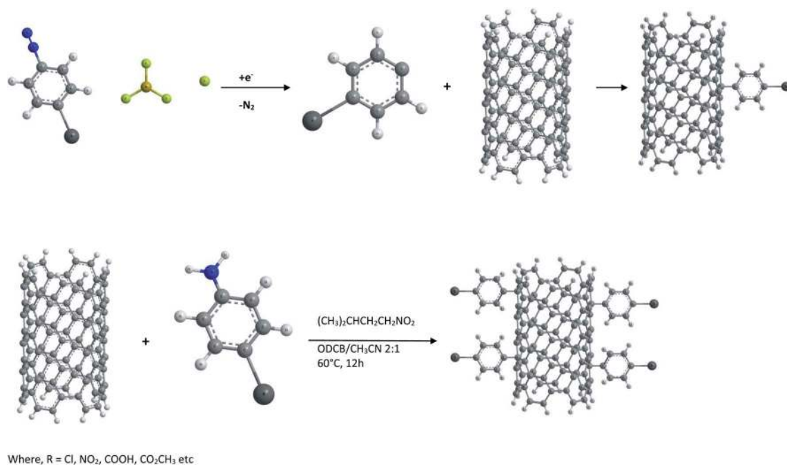
Fig. 2 Arylation of CNTs via reduction of diazonium salts, where R = Cl, NO 2 , COOH, CO 2 CH 3 etc.
