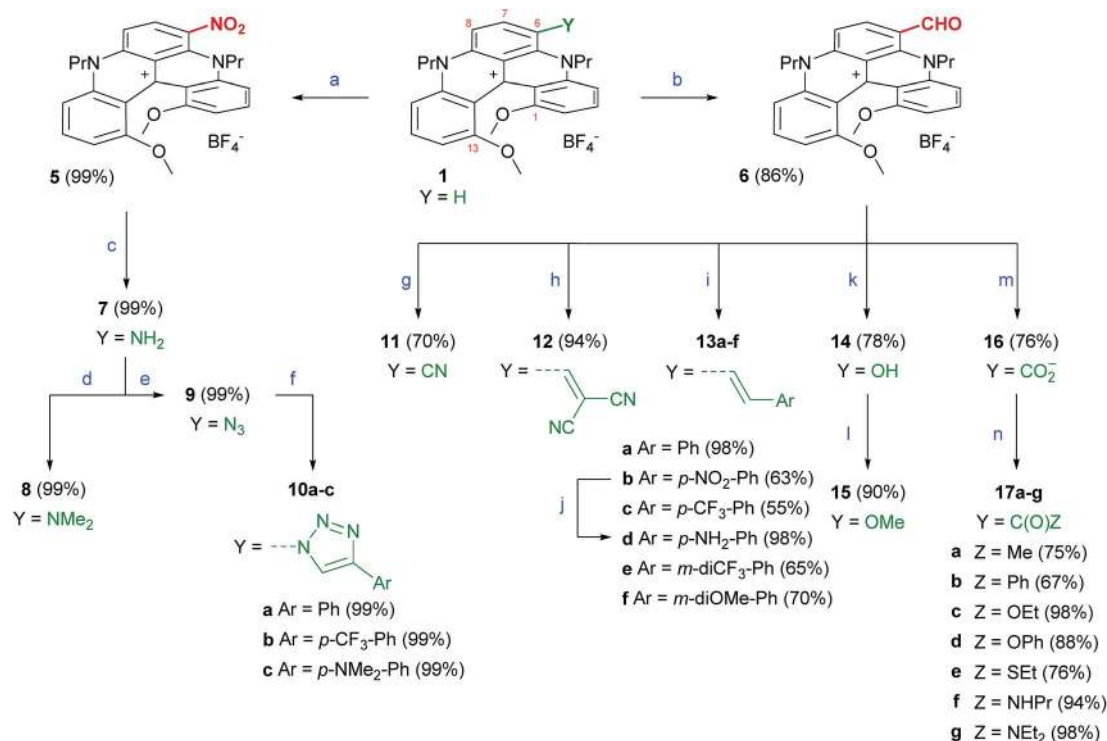
Scheme 1 Synthesis of functionalized [4]helicenes. Reagents and conditions: (a) HNO_3 (60% aq.), CH_2Cl_2 , 25 °C, 15 min. (b) POCl_3 , DMF, 90 °C, 8 h. (c) H_2 , Pd/C (0.2 equiv.), CH_2Cl_2/MeOH , 25 °C, 1 h. (d) (i) HCHO (12 equiv.), NaBH_3CN (7 equiv.), THF, 25 °C, 30 min; (ii) AcOH , 3 h; (iii) NaOH ; (iv) 1 M aq. HBF_4 . (e) tBuONO (1.5 equiv.), TMSN_3 (1.2 equiv.), MeCN, 0 to 25 °C, 3 h. (f) ArC\equiv CH , CuSO_4 \cdot 5H_2O (0.2 equiv.), ascorbic acid (0.3 equiv.), NaHCO_3 (0.3 equiv.), MeCN/ H_2O , 25 °C, 12 h. (g) NaN_3 (1.5 equiv.), TfOH (3 equiv.), MeCN, 25 °C, 10 min. (h) NCCH_2CN (3 equiv.), Ph_3P (20 mol%), MeCN, 130 °C (MW), 25 °C, 1 h. (i) (i) ArCH_2X (1.2 equiv.), Ph_3P (1.3 equiv.), CH_2Cl_2 ; (ii) NaH (2 equiv.), DCM, 25 °C, 30 min; (iii) 1 M aq. HBF_4 . (j) AcOH (15 equiv.), Zn (5 equiv.), CH_2Cl_2 , 25 °C, 3 h. (k) mCPBA (5 equiv.), CH_2Cl_2 , 25 °C, 2 h. (l) Mel (3 equiv.), K_2CO_3 (5 equiv.), MeCN, reflux, 1 h. (m) NaH_2PO_4 (1 equiv.), NaClO_2 (2 equiv.), H_2O_2 , MeCN, 60 °C, 1 h. (n) (i) SOCl_2 (6 equiv.), CH_2Cl_2 , 25 °C, 10 min; (ii) for 17a,b : MeMgI or PhMgI (1.5 equiv.), -5 °C, 30 min, then 1 M aq. HBF_4 ; for 17c,e : EtOH , PhOH or EtSH (5 or 15 equiv.), 25 °C, 10 min or 2 h; for 17f,g : PrNH_2 or Et_2NH (15 equiv.), 0 °C then 25 °C, 15 min.
