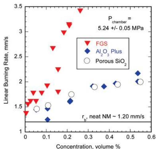
Figure 6. Linear burning rate of nitromethane and catalyst support additive mixtures as a function of volume concentration (density of FGS assumed to be 2.17 \text{ g/cm}^3 ). The burning rate of neat NM is estimated using the experimentally derived correlation from Boyer and Kuo. 34
