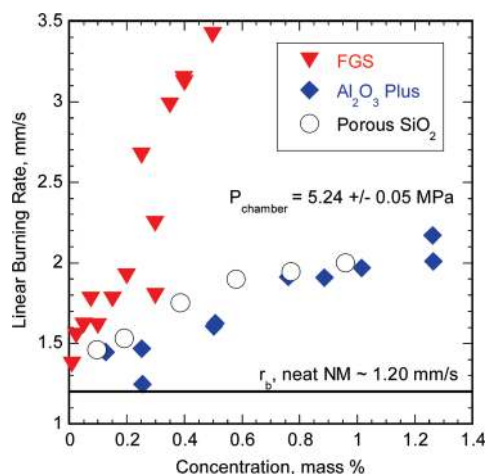
Figure 5. Linear burning rate of nitromethane and catalyst support additive mixtures as a function of mass concentration. The burning rate of neat NM is estimated using the experimentally derived correlation from Boyer and Kuo. 34
