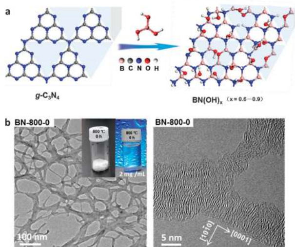
Fig. 2 (a) Preparation of hydroxylated BNs through thermal substitution of carbon atoms in g\text{-C}_3\text{N}_4 using boric acid. (b) Low- (left) and high-resolution (right) TEM images of the precipitated hydroxylated BN materials extracted from an aqueous solution. The sample is prepared at 800\text{ }^\circ\text{C} . The insets in (b) are the photographs of the as-prepared hydroxylated BN and its aqueous solution with a concentration of 2\text{ mg mL}^{-1} . Reproduced from ref. 70 with permission.
