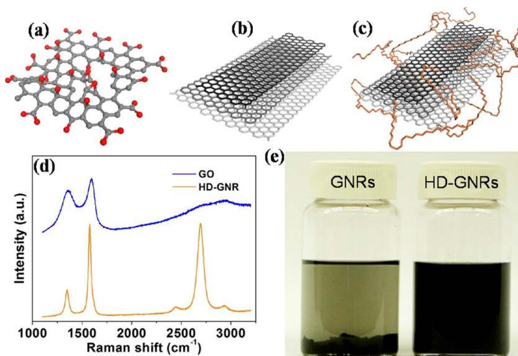
Figure 1. Chemical structure of (a) GO, (b) GNRs, (c) HD-GNRs, (d) Raman spectra of GO and HD-GNRs; (e) dispersion study of GNRs (left) and HD-GNRs (right) in chloroform (1 mg/mL).
