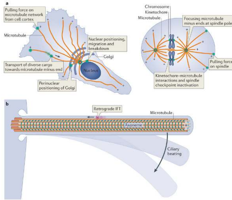
Figure 1. Sites of dynein action in the cell
