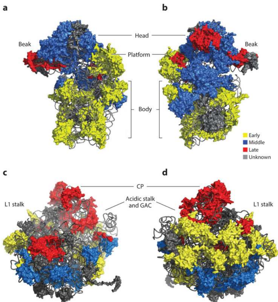
Figure 3. Correlation of function and location of the small subunit (SSU) and large subunit (LSU) r-proteins of Saccharomyces cerevisiae . Early-acting (yellow), middle-acting (blue), and late-acting (red) r-proteins are mapped onto the crystal structure. (a,c) The subunit interface of the SSU and LSU, respectively. (b,d) The solvent-exposed surface of the SSU and LSU, respectively. Ribosomal RNA (rRNA) and r-proteins are shown in cartoon and surface representation, respectively. Abbreviations: CP, central protuberance; GAC, GTPase-activation center. The crystal structure is adapted from Protein Data bank codes 3U5D and 3U5E.
