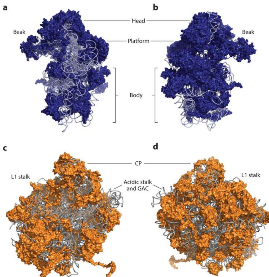
Figure 1. Crystal structure of (a,b) the small subunit (SSU) and (c,d) the large subunit (LSU) from Saccharomyces cerevisiae at 3.0-Å resolution. (a,c) The subunit interface of the SSU and LSU, respectively. (b,d) The solvent-exposed surface of the SSU and LSU, respectively. Abbreviations: CP, central protuberance. GAC, GTPase-activation center. The crystal structure is adapted from Protein Data Bank codes 3U5B, 3U5C, 3U5D, and 3U5E.
