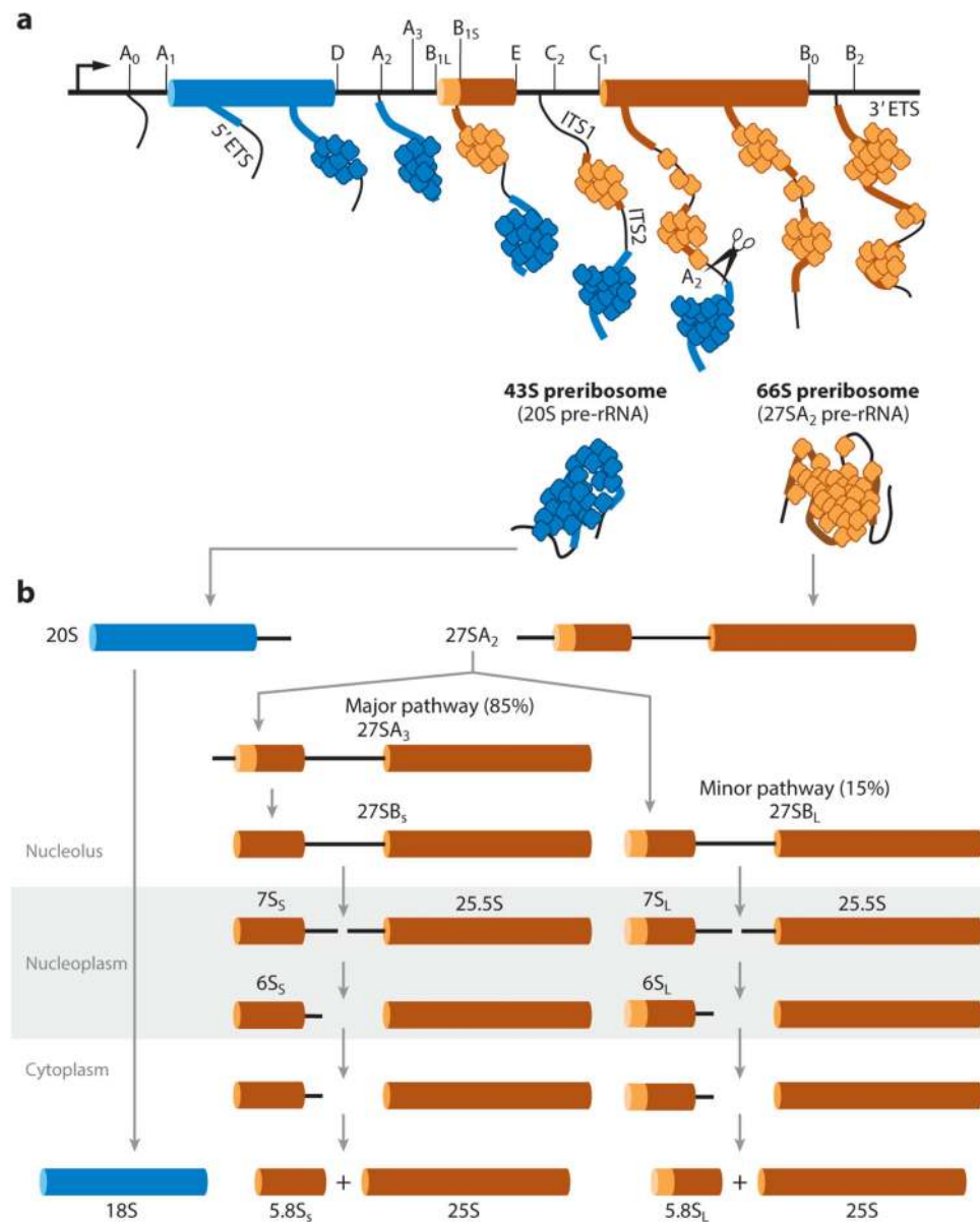
Figure 2. Cotranscriptional precursor rRNA (pre-rRNA) processing in Saccharomyces cerevisiae . (a) As RNA polymerase I transcribes a ribosomal DNA (rDNA) repeat, nascent pre-rRNAs are cleaved cotranscriptionally at the A 2 site, releasing a 43S preribosome containing 20S pre-rRNA. The 66S preribosome containing 27SA 2 pre-rRNA is released upon completion of transcription. The pre-rRNA processing sites are indicated along the rDNA gene, and the external and internal transcribed spacer sequences are indicated on the nascent transcript. (b) The pre-rRNAs then undergo a series of exo- and endonucleolytic cleavages to remove the spacer sequences, finally liberating mature 18S, 5.8S, and 25S rRNAs. Not shown is the flanking 5S gene, transcribed in the opposite direction.
