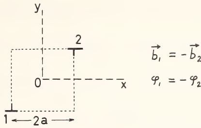
FIGURE 7. Dislocation dipole.
