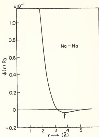
FIGURE 1. Pair interactions between two sodium ions. Energy is measured in Rydbergs and separation in Å. The arrow indicates the nearest neighbor distance observed in the b.c.c. phase.
