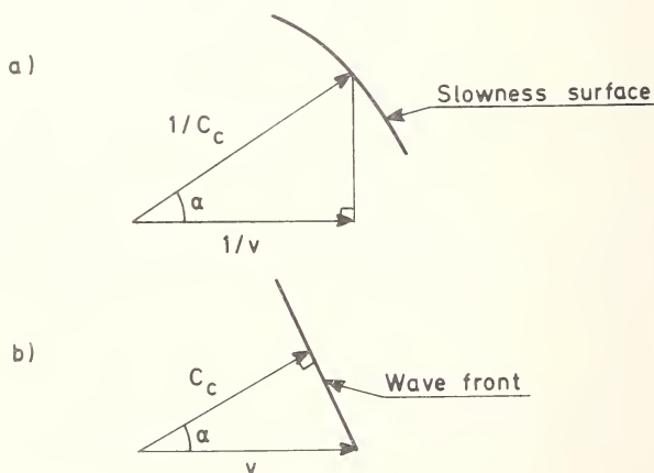
FIGURE 6. Comparison of Čerenkov wave velocity C_c constructed from a) slowness surface b) wave front
