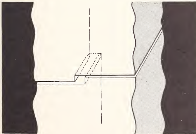
FIGURE 2. The figure shows how a kink is created by cutting a screw dislocated crystal perpendicular to the line of the screw, and displacing the two halves of the crystal in the plane of the cut. The extra "half plane" of atoms for the kink which results is manifested as the empty slot into which new material must be inserted.
