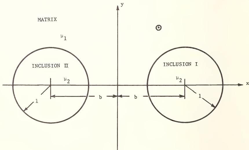
FIGURE 2. Screw dislocation \odot near two equal inclusions of unit radius.
