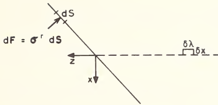
FIGURE 5. A dislocation loop \delta x \delta \lambda in a half infinite medium.
