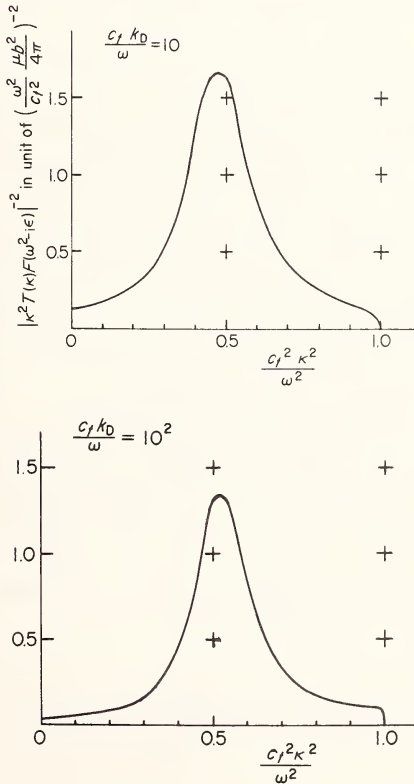
FIGURE 6. A plot of |\kappa^2 T(\kappa) F(\omega^2 - i\epsilon)|^{-2} for a screw dislocation in an isotropic medium as a function of \kappa . (c_l/c_l)^2 is assumed to be 1/3 (Cauchy relation).
