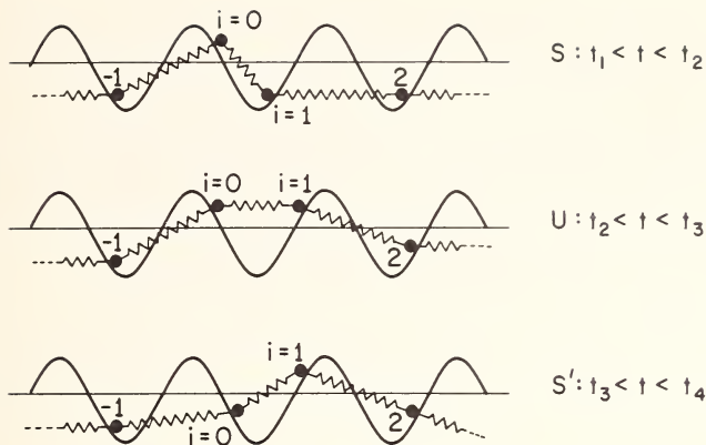
FIGURE 2. Sequence of atom positions during dislocation motion.
