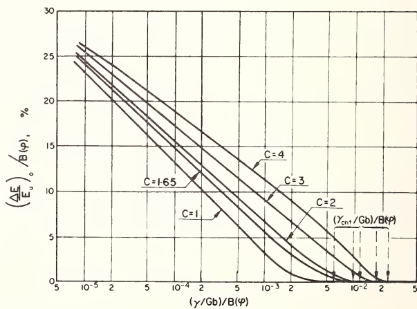
FIGURE 2. The relative energy gain due to the extension of 1/2 \langle 110 \rangle , \{111\} dislocations into Shockley partials, (\Delta E/E_n)_0 , as a function of the stacking fault parameter \gamma/Gb . The function B(\phi) , representing the dependence on relative dislocation orientation, is given by eq (11b).
