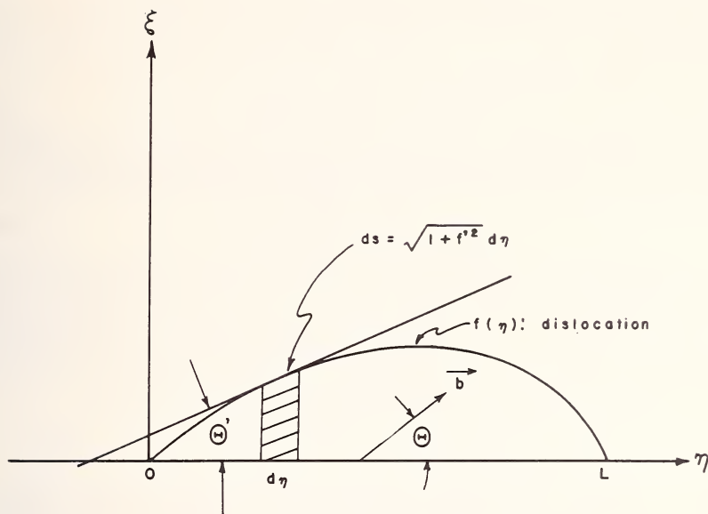
FIGURE 1. Bowed-out dislocation \xi=f(\eta) . \eta axis coincides with the straight-line configuration of the dislocation before bowing out. \mathbf{b} , Burgers vector.
