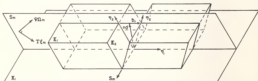
FIGURE 1. Twinning elements in crystals. \kappa_1 is the twin plane and \eta_1 the shear direction. \kappa_2 and \eta_2 are the elements for the second undistorted plans. S_m is the plane of shear containing \Psi\Omega_m and T\xi_m orthogonal unit vectors.
