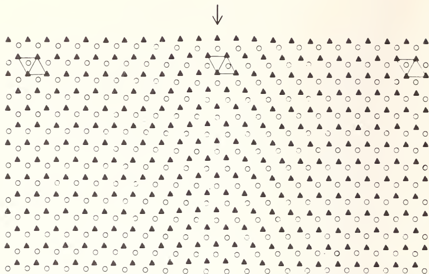
FIGURE 1. Positions of atoms in two \{111\} planes, one above, \blacktriangle , and one below, \circ , the slip plane of a dissociated edge dislocation. The region of stacking fault which separates partial dislocations can easily be distinguished by observing the figure from either side at a low angle.
