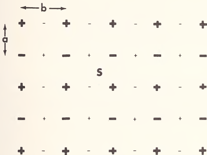
FIGURE 5. Schematic drawing of the ion positions on the [110] plane of NaCl with lattice parameters a and b . The screw emerges at S . The ledge caused by the screw can run in either the [001] direction (vertical) or in the [110] direction (horizontal). The heavy ions are the surface ions; the light ones are those lying a distance b/2 below the surface. When a quarter plane is added to turn a vertical ledge into a horizontal one, \pm e/4 is added to the screw emergent point.
