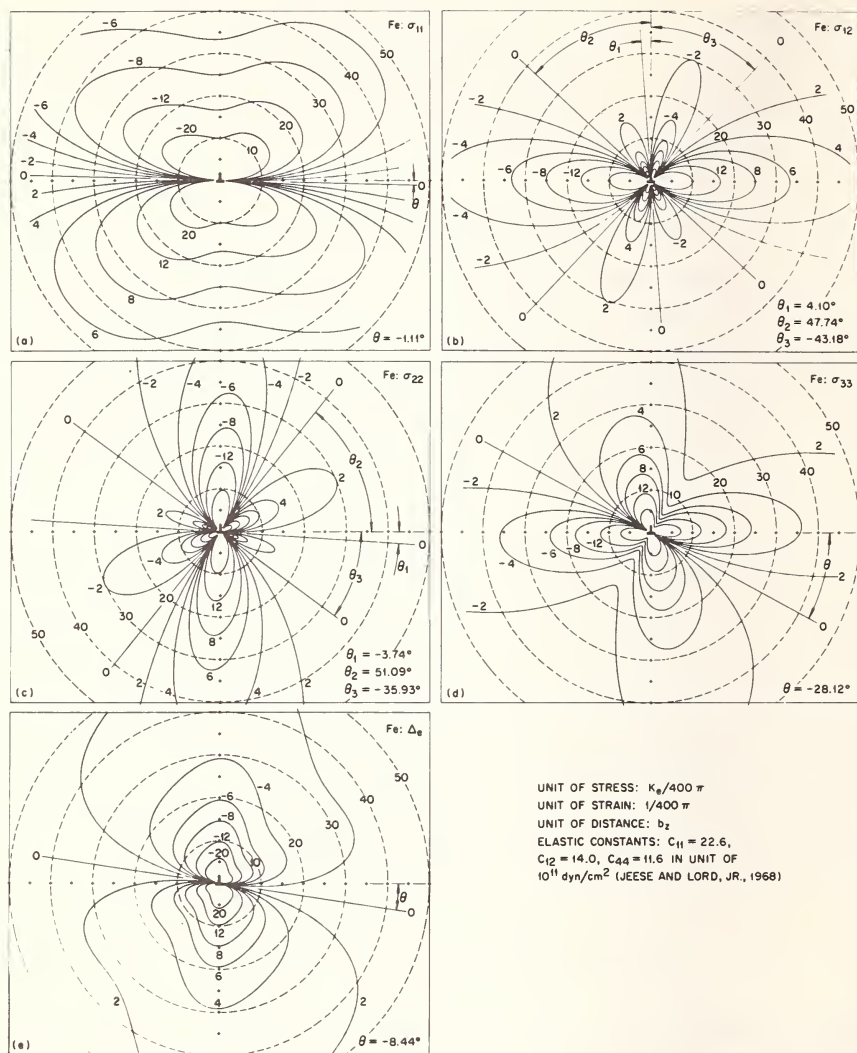
FIGURE 4. Stress fields and dilation field of an edge twin dislocation. \{112\} \langle 11\bar{1} \rangle twin of Fe.
