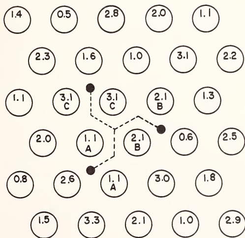
FIGURE 1. Atom arrangement of screw dislocation in b.c.c. iron viewed along the dislocation line. The dislocation a/2 [111] dissociates into three partials with the Burgers vector a/6 [111]. The stacking faults are shown by broken lines. (Based on the calculation by Chang [12])
