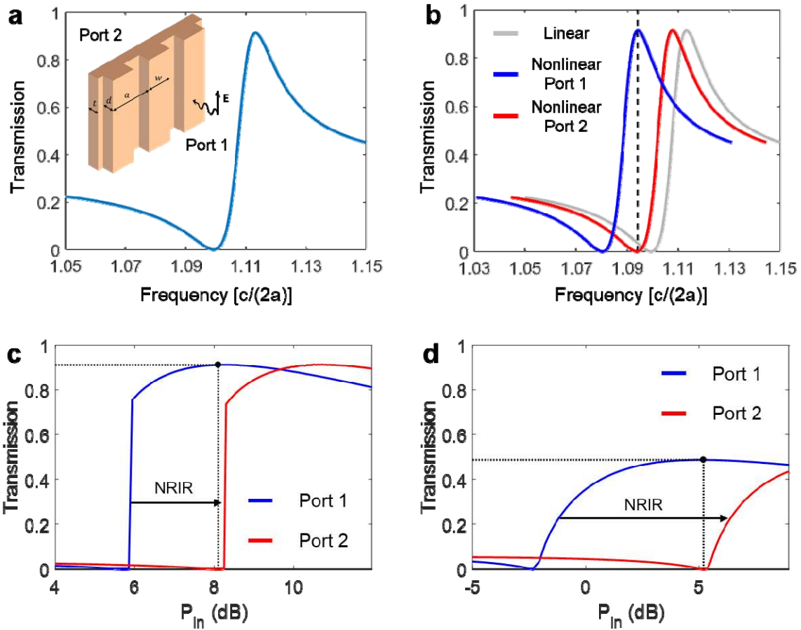
Figure 1. Nonlinear Fano isolator based on a substrate-backed dielectric grating. (a) Linear response and schematic of the structure for d = 0.1a , w = 0.8a , t = 0.03a and \epsilon_{lin} = 12 . (b) Desired nonlinear response, for which a transmission maximum from port 1 is aligned in terms of input intensity with a zero from port 2. The vertical dashed line indicates the excitation frequency. (c) Actual nonlinear response for the same parameters as in panel (a), excitation frequency f = 1.094c/(2a) and third-order nonlinear susceptibility \chi^{(3)} = 2.8 \times 10^{-18} \text{ m}^2/\text{V}^2 . (d) Similar to panel (c) but for t = 0.08a and f = 0.9575c/(2a) . The numerical results were derived through full-wave simulation with Comsol Multiphysics.
