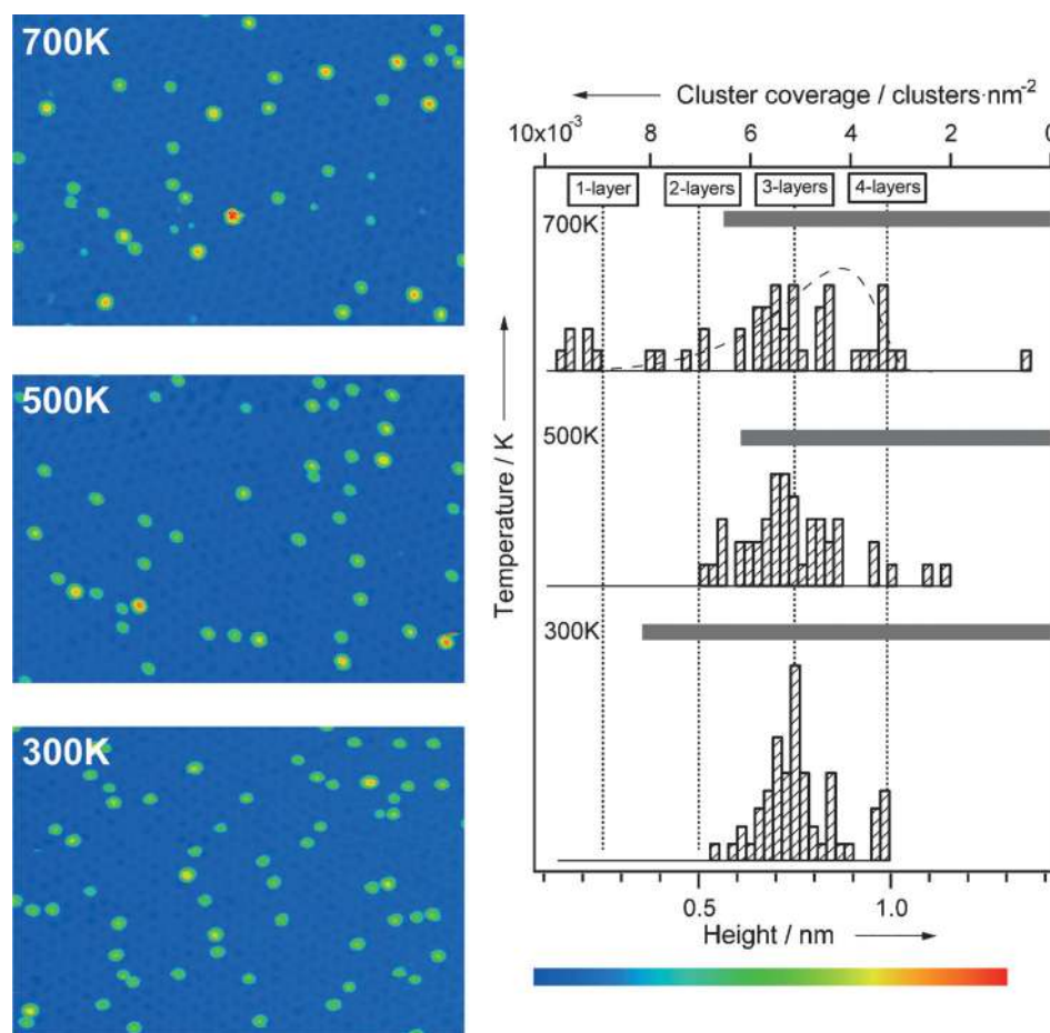
Figure 6. Left: Ripening of Pd 19 clusters on a h-BN/Rh(111) surface upon sample annealing for 5 min at the indicated temperature. Image size: 75 \times 100 nm 2 ; imaging conditions: +1.0 V, 1 pA. Right: Bottom axis: Particle-size distributions that correspond to the images on the left. The PSDs are obtained as height histograms, normalized to the relative frequencies. As a guide to the eye, the 700 K data are fitted to the model of Finsy. [10] Top axis: Observed cluster coverage at each annealing temperature, as represented by gray bars. The cluster coverage does not decrease as much as for the graphene-Moiré samples. The broadening of the PSDs, without a shift, and the almost-constant cluster coverage indicate an OR mechanism.
