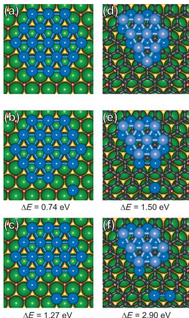
Figure 3. Optimized atomic configurations that were obtained from first-principles DFT calculations for \text{Pd}_{19} clusters on bare Rh(111) (a–c) and on g/Rh(111) (d–f). Starting from the most-stable configurations (a, d), we show the atomic configurations that correspond to the lowest-energy single atom (b, e) and their related dimer-detachment processes (c, f). The single-atom detachment process on Rh(111) entails a transition-state barrier of 0.89 eV, which is encountered 0.6 Å prior to reaching the local-energy minimum shown in (b); overall the atom covers in this detachment process a distance of 2.55 Å with respect to the initial configuration, and the final configuration is 0.74 eV higher in energy. The corresponding detachment of a Pd dimer entails a total energy increase of 1.27 eV (c). In contrast, the single-atom detachment process on g/Rh(111) leads to an atom displacement of 2.63 Å prior to reaching the local-energy minimum shown in (e); the final configuration is 1.50 eV higher in energy, which is twice the value for single-atom detachment from the cluster that is adsorbed on the bare Rh(111) surface. The detachment of a Pd dimer from the \text{Pd}_{19} cluster on g/Rh(111) even entails an overall energy increase of 2.90 eV (f). For the color legend, see Figure 2.
