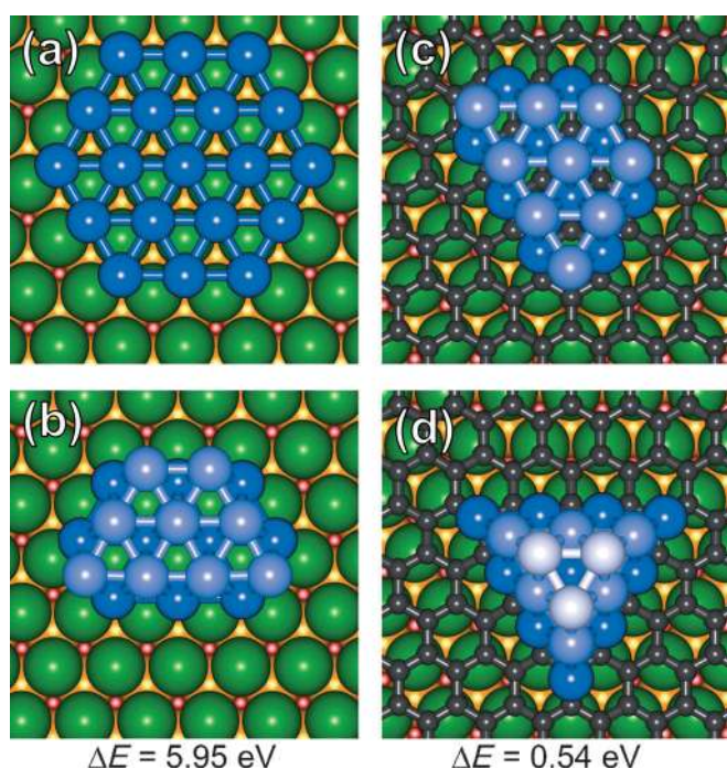
Figure 2. Optimized atomic configurations that were obtained from first-principles DFT calculations for \text{Pd}_{19} clusters on bare Rh(111) (a,b) and on g/Rh(111) (c,d). On Rh(111), the most-stable configuration is the 2D (one-layer) configuration (a), whereas the 3D (two-layer) configuration is 5.95 eV higher in energy (b). On the r-hcp sites of g/Rh(111), 3D structures are preferred, with a most-stable configuration of 2 layers (c), whereas the three-layer configuration is only 0.54 eV higher in energy (d). Rh substrate atoms are depicted by large green (first layer), orange (second layer), and red spheres (third layer). Carbon atoms of the graphene-Moiré film are depicted as small dark-gray spheres (c,d). Pd cluster atoms in direct contact with the underlying surface are depicted as dark-blue, light-blue (second cluster layer, b–d), and whitish-blue spheres (third cluster layer, d).
