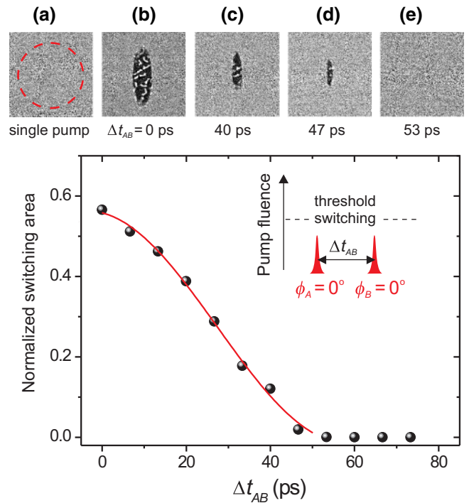
FIG. 2. Photomagnetic “write-write” sequence with two identical pulses linearly polarized along the [100] ( \phi_A = \phi_B = 0^\circ ) crystallographic axis. The fluence is 25% less than the minimum required for single-pulse switching (see inset). The magneto-optical difference images (top panel) show the laser-induced changes of domain structure after excitation with (a) single A (or B ) pulse, (b) fully overlapping A and B pulses ( \Delta t_{AB} = 0 ps), (c)–(e) separated pulses when pulse B arrives after pulse A . The plot shows the switched area as a function of delay time between A and B pulses. The solid red line is a fit with \cos(2\pi \Delta t_{AB}/T) function where T/2 = 62 \pm 1 ps. The fitting range is limited to the range with nonzero values of normalized switching area.
