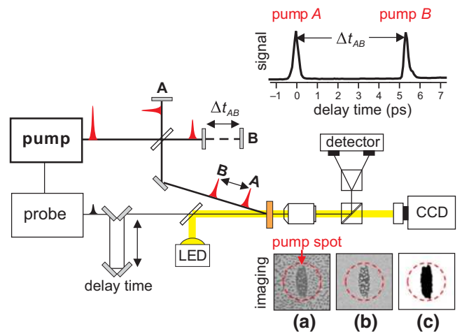
FIG. 1. The geometry of the double-pump experiment. Two pump laser pulses labeled “A” and “B” with the central wavelength \lambda = 1300 nm and controlled polarizations are used to trigger magnetization precession or switching (a). The separation time \Delta t_{AB} between the two pump pulses is the experimental variable. The pump pulses are obtained via splitting the initial laser pulse in an interferometer. The separation time between the pumps can be varied by changing the length of one of the arms. The normalized switched area is calculated as the ratio of the recorded domain area [the large black domain in Fig. 1(c)] to the area of the laser spot \pi d^2/4 (spot is shown by dashed red circle). (b) Magneto-optical difference image between images obtained after and before the double-pump excitation. The size of the images is 200 \times 200 \mu\text{m}^2 .
