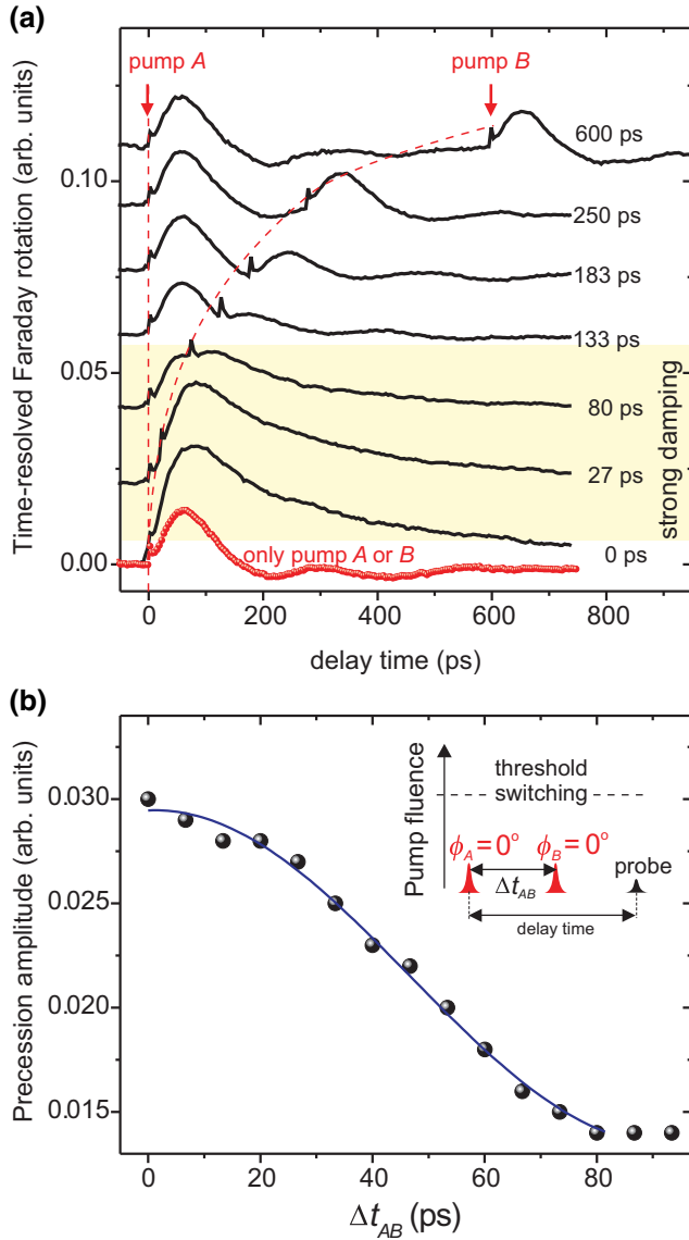
FIG. 3. Time-resolved magneto-optical Faraday rotation induced by two weak “write”-“write” pulses linearly polarized along [100] axis ( \phi_A = \phi_B = 0^\circ ) with intensities of 8 \text{ mJ/cm}^2 . Even fully overlapping pump pulses cannot write a domain. (a) Shows time traces of the magneto-optical signal measured for different delays between the pump pulses \Delta t_{AB} . The filled red circles show magnetization dynamics for single pump A pulse. Pulse B alone triggers the same dynamics. The curves are shifted vertically without rescaling of the plots. (b) Shows the amplitude of magnetization precession as a function of \Delta t_{AB} deduced from data on panel (a). The solid blue line is a fit with \cos(2\pi \Delta t_{AB}/T) function where T/2 = 91 \pm 4 \text{ ps} . The fitting is limited to the range where the amplitude of the oscillations triggered by two pulses exceeds the amplitude of the oscillations triggered by pulse A alone.
