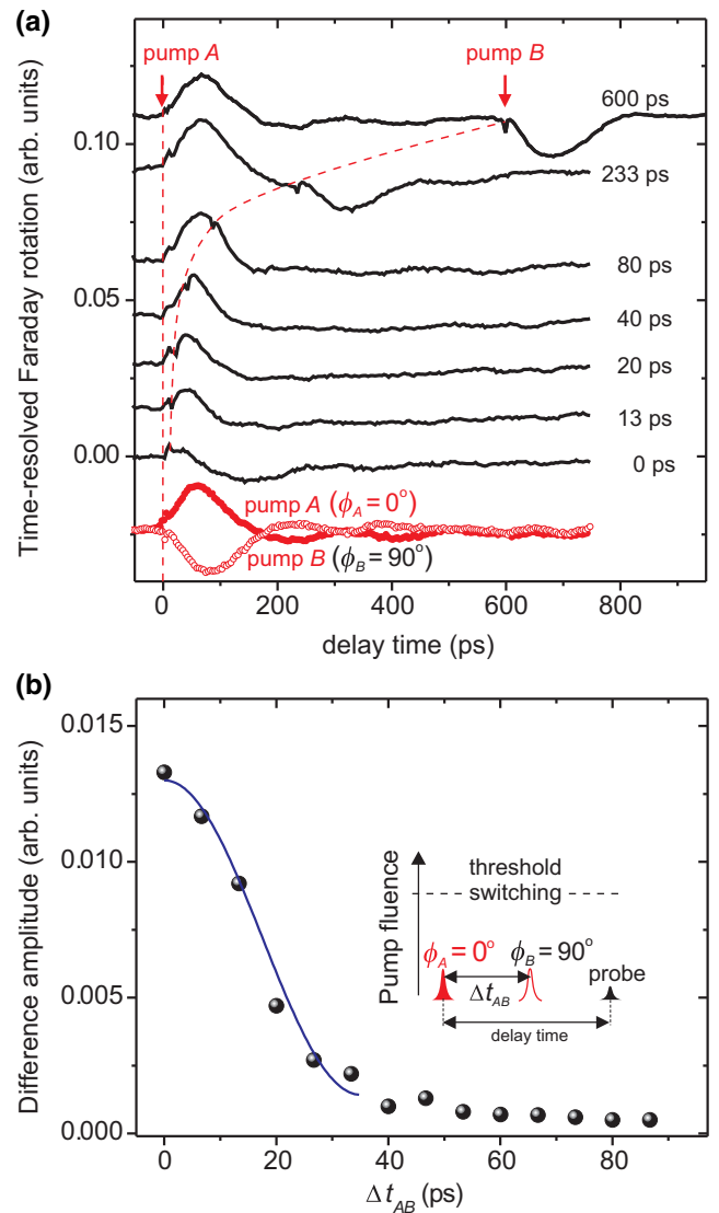
FIG. 5. Time-resolved magneto-optical Faraday rotation induced by two weak “write-erase” pulses. The write pulse is linearly polarized along the [100] ( \phi_A = 0^\circ ) axis, while the erase pulse is polarized along the [010] ( \phi_B = 90^\circ ). The pulse intensities are 8 \text{ mJ/cm}^2 , that is, at the level of 25% of the minimum fluence required for the switching. (a) Shows time traces of the magneto-optical signal measured at different delays between the pump pulses \Delta t_{AB} . The filled red circles show magnetization dynamics for single pump pulse A . Pulse B alone triggers the same dynamics. The curves are shifted vertically without rescaling of the plots. (b) Shows the difference between the amplitudes of the oscillations triggered by the double-pulse excitation and pulse A only. The solid blue line is a fit using \cos(2\pi \Delta t_{AB}/T) function where T/2 = 35 \pm 3 ps.
