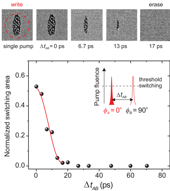
FIG. 4. The effect of a write-erase sequence. Top panel – magneto-optical difference images obtained after pumping with two pulses at different times of pump-pulses separation. The write-pulse A is linearly polarized along the [100] crystallographic axis ( \phi = 0^\circ ). The erase pulse B is linearly polarized along the [010] axis ( \phi_B = 90^\circ ). The graph shows the efficiency of switching as a function of separation between two pump pulses. The solid red line is a fit using \cos(2\pi \Delta t_{AB}/T) function where T/2 = 18 \pm 5 ps. Fitting is limited to the range with nonzero values of normalized switching area.
