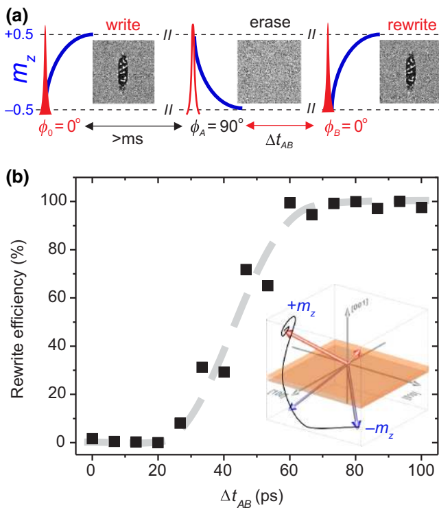
FIG. 6. The effect of write-erase-write sequence. (a) Magneto-optical difference images obtained after pumping with three pulses. After a domain is written by “0” pump, the medium is excited by a sequence of erase-write ( A - B ) pulses. The experiments are performed for a different time of separation between A and B pulses \Delta t_{AB} . The “0” pump write pulse is linearly polarized along the [100] crystallographic axis ( \phi_0 = 0^\circ ). The erase-pulse A is linearly polarized along the [010] axis ( \phi_B = 90^\circ ). The write pulse B is linearly polarized along the [100] axis. (b) Efficiency of switching as a function of separation between pump pulses’ separation. The dashed red line is a guide to the eye. The inset (b) shows the trajectory of magnetization switching calculated using the model from Ref. [17].
