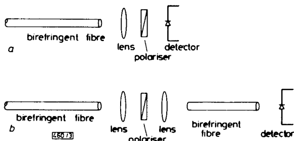
Fig. 3 Performance of bulk polarisers as y -polarised mode selector
