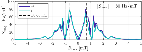
(b) Magnetic sensitivity S_{\text{mag}} as a function of the external magnetic bias flux density B_{\text{bias}}
