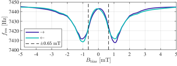
(a) Resonance frequency f_{\text{res}} as a function of the external magnetic bias flux density B_{\text{bias}}
