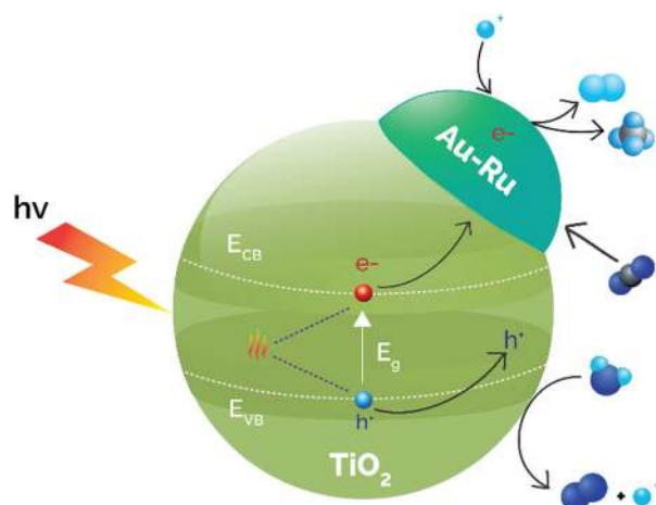
Fig. 9 Synergistic effects between photocatalysis and thermocatalysis in the direct thermophotocatalytic reduction of CO 2 –H 2 O over Au–Ru/TiO 2 . Adapted with permission from ref. 159. Copyright (2017) John Wiley and Sons.
