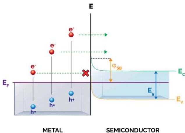
Fig. 3 Schematic illustration of the metal/semiconductor Schottky barrier. Upon excitation, only hot electrons with enough energy can surpass the Schottky barrier ( \varphi_{\text{SB}} ) and transfer into the conduction band of the semiconductor.
