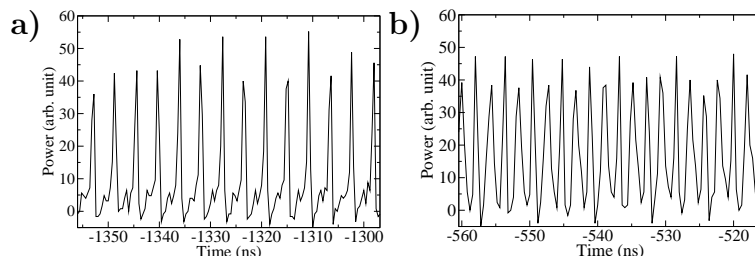
Fig. 19. Close-up of timetraces of a switch-on transient recorded with a fast avalanche photodiode located at the position of the stationary LCS. The zero of the time axis is arbitrary. a) is obtained in the beginning of the transient, b) later on. [Reprinted figure with permission from Tanguy et al. (2008a). Copyright 2008 of the American Physical Society.]
