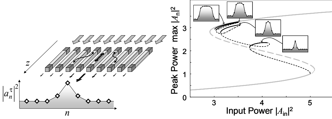
Fig. 29. Left side: Coupled cavities formed by a waveguide array with mirrors on each end facets. Right side: Stability range of discrete SDS for the defocusing case. Homogeneous solution (grey curve, solid for stable, dashed for unstable, dotted for modulationally unstable), peak power of discrete SDS (black curve, solid for stable and dashed for unstable). The insets show discrete SDS of different orders. Parameters are \alpha = -1 , \Delta = 2.5 and C = 0.25 . [Reprinted figures with permission from Peschel et al. (2004). Copyright 2004 by the Optical Society of America. ]
