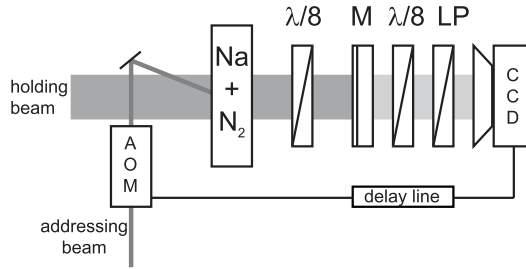
Fig. 33. Schematic experimental setup. \lambda/8 : \lambda/8 retardation plate, M: mirror of high reflectivity, LP: linear polarizer, CCD: charge-coupled device camera, AOM: acousto-optic modulator
