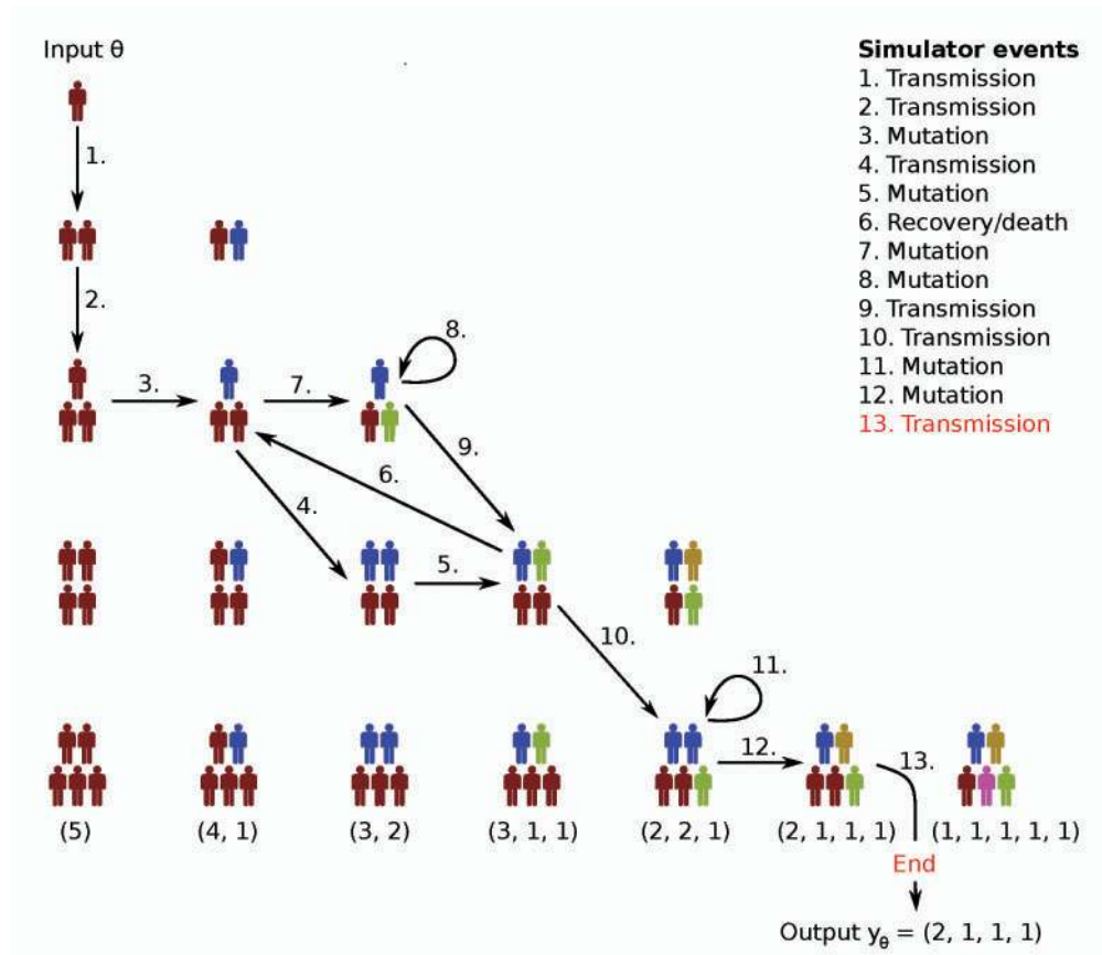
FIGURE 2. An example of a transmission process simulated under a parameter configuration \theta without subsampling of the simulated infectious population. Arrows indicate the sequence of random events taking place in the simulation and different colors represent different haplotypes of the pathogen. The simulation starts with one infectious host who transmits the pathogen to another host. After one more transmission event, the pathogen undergoes a mutation within one of the three hosts infected so far (event three). As the sixth event in the simulation, one of the haplotypes is removed from the population due to the recovery/death of the corresponding host. The simulation stops when the infectious population size exceeds m=5 and the simulator outputs the generated y_\theta . The nodes not connected by arrows show all the other possible configurations of the infectious population, but which were not visited in this example run of the simulator. The bottom row lists the possible outputs of the simulator (cluster size vectors) under their corresponding population configuration.
