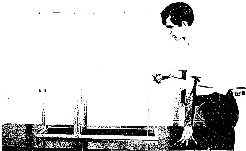
Figure 2. This device was designed by students and built by the departmental technician. The apparatus employs a pendulum that can be used to illustrate the impact resistance of planar composite materials.
