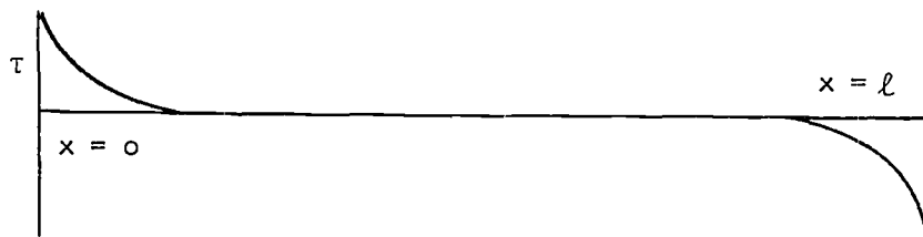
Figure E-4. The Variation of Shear Stress, \tau , Along a Fiber of Length \ell , According to Equation (16).
