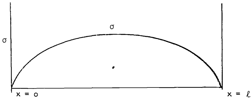
Figure E-3. The variation of Tensile Stress, \sigma , along a Fiber of Length, l , According to Equation (5).
