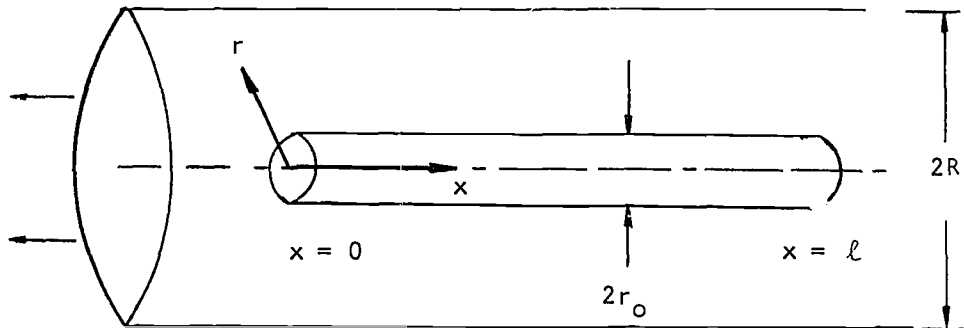
Figure E-2. A Long, Thin, Straight Fiber Completely Embedded in a Continuous, Homogeneous Matrix. (Elastic-Elastic System)
