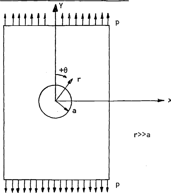
Circular Hole in a Loaded Plate
