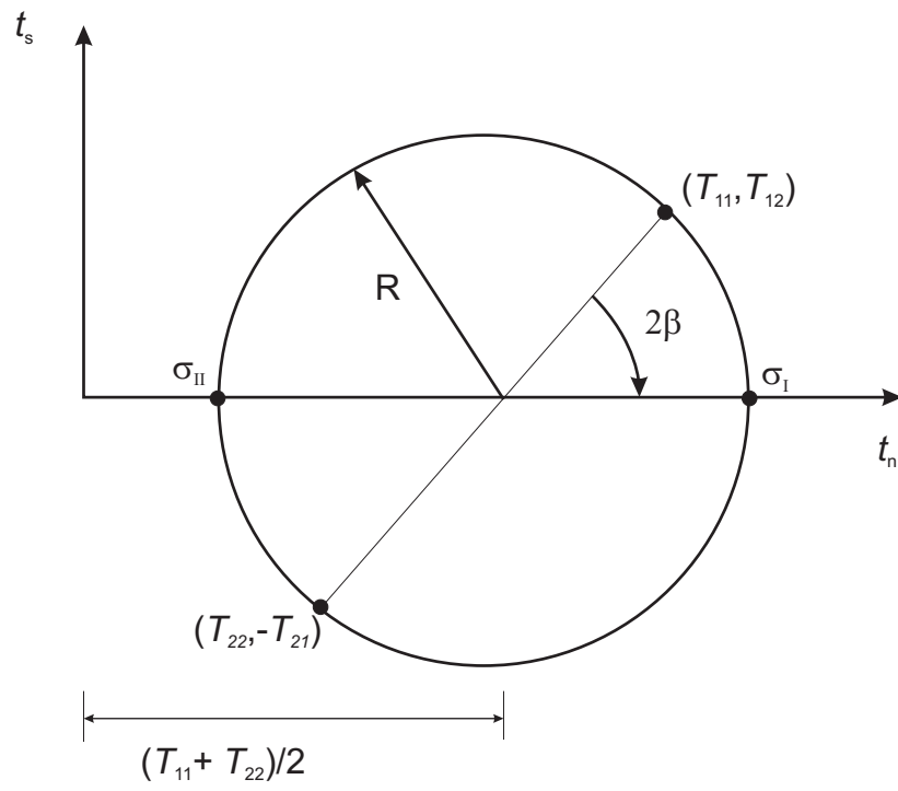
Figure 14.3: Mohr's circle.
